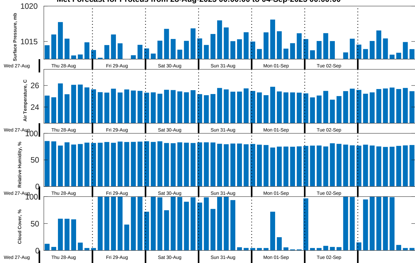
Met Forecast for Proteus from 28-Aug-2025 00:00:00 to 04-Sep-2025 00:00:00
