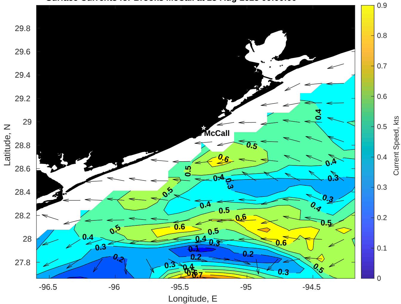
Surface Currents for Brooks McCall at 28-Aug-2025 00:00:00
