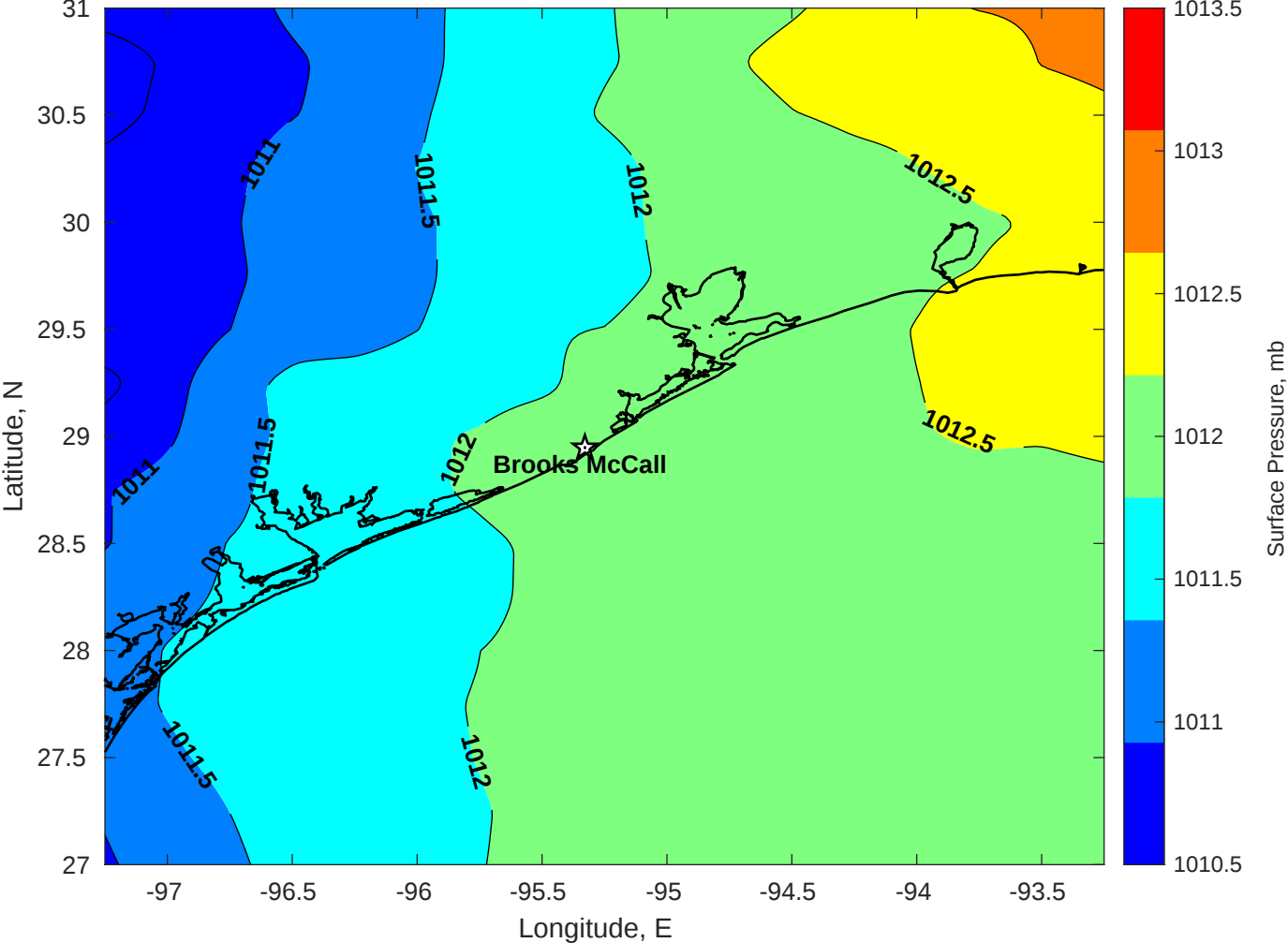
Surface Pressure (mb) for Brooks McCall at 31-Aug-2025 00:00:00
