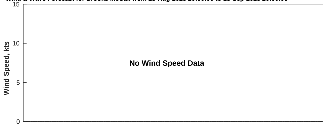
Wind & Wave Forecast for Brooks McCall from 28-Aug-2025 20:00:00 to 13-Sep-2025 20:00:00
