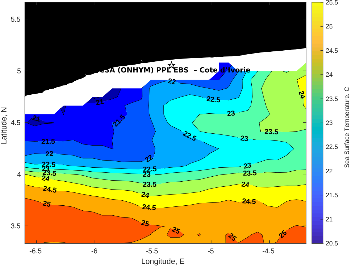
SST for CSA (ONHYM) PPL EBS - Cote d'Ivoire at 28-Aug-2025 00:00:00
