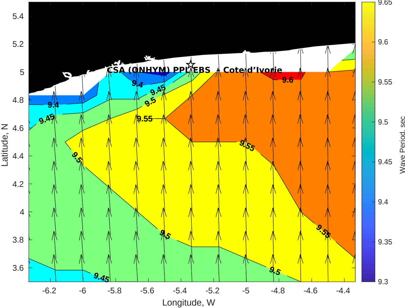
Wave Period (sec) for CSA (ONHYM) PPL EBS - Cote d'Ivoire at 29-Aug-2025 09:00:00
