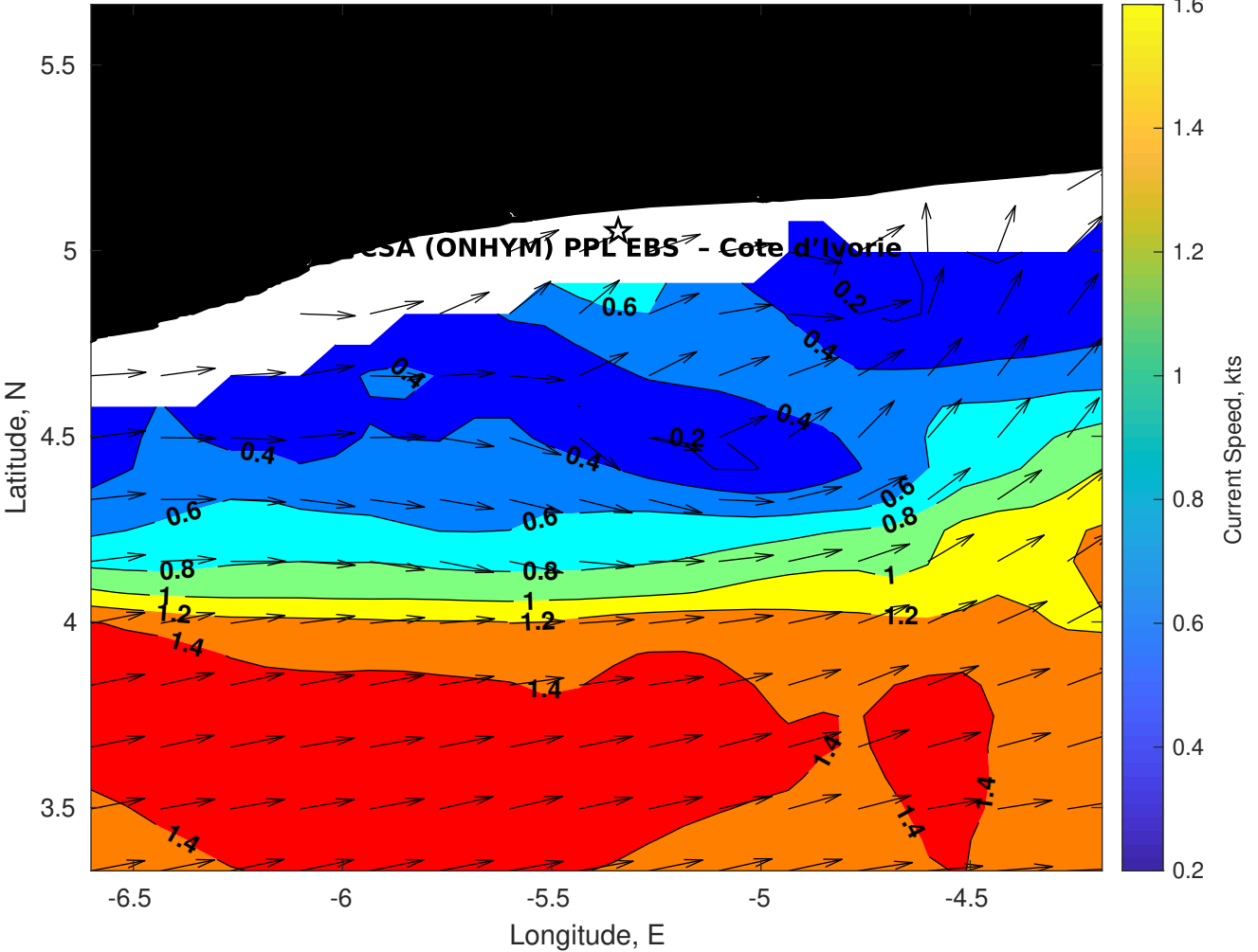
Surface Currents for CSA (ONHYM) PPL EBS - Cote d'Ivoire at 28-Aug-2025 00:00:00
