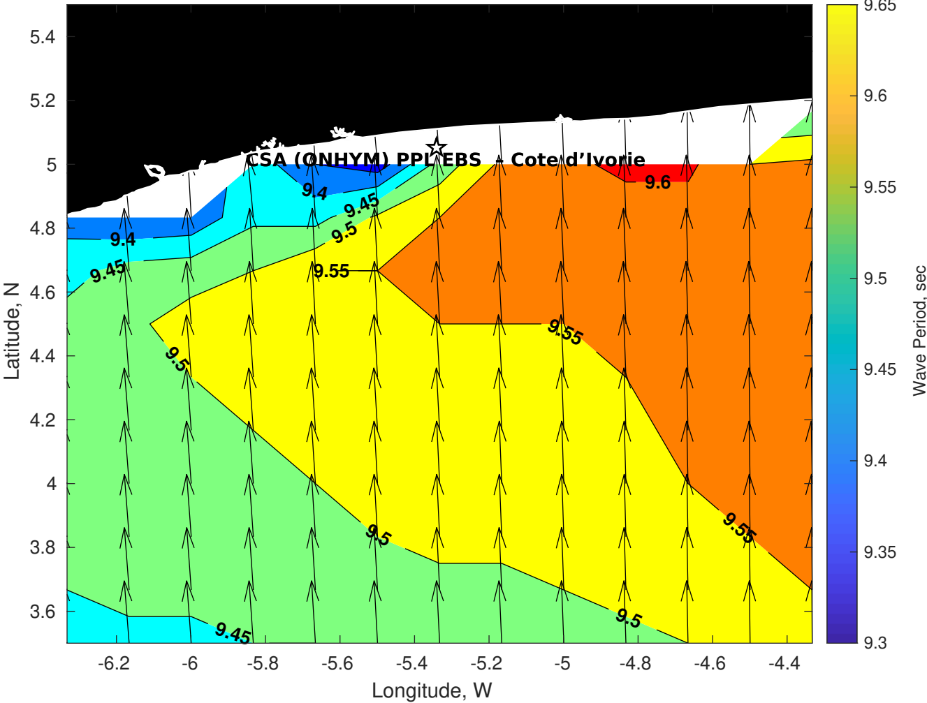
Wave Period (sec) for CSA (ONHYM) PPL EBS - Cote d'Ivoire at 29-Aug-2025 09:00:00
