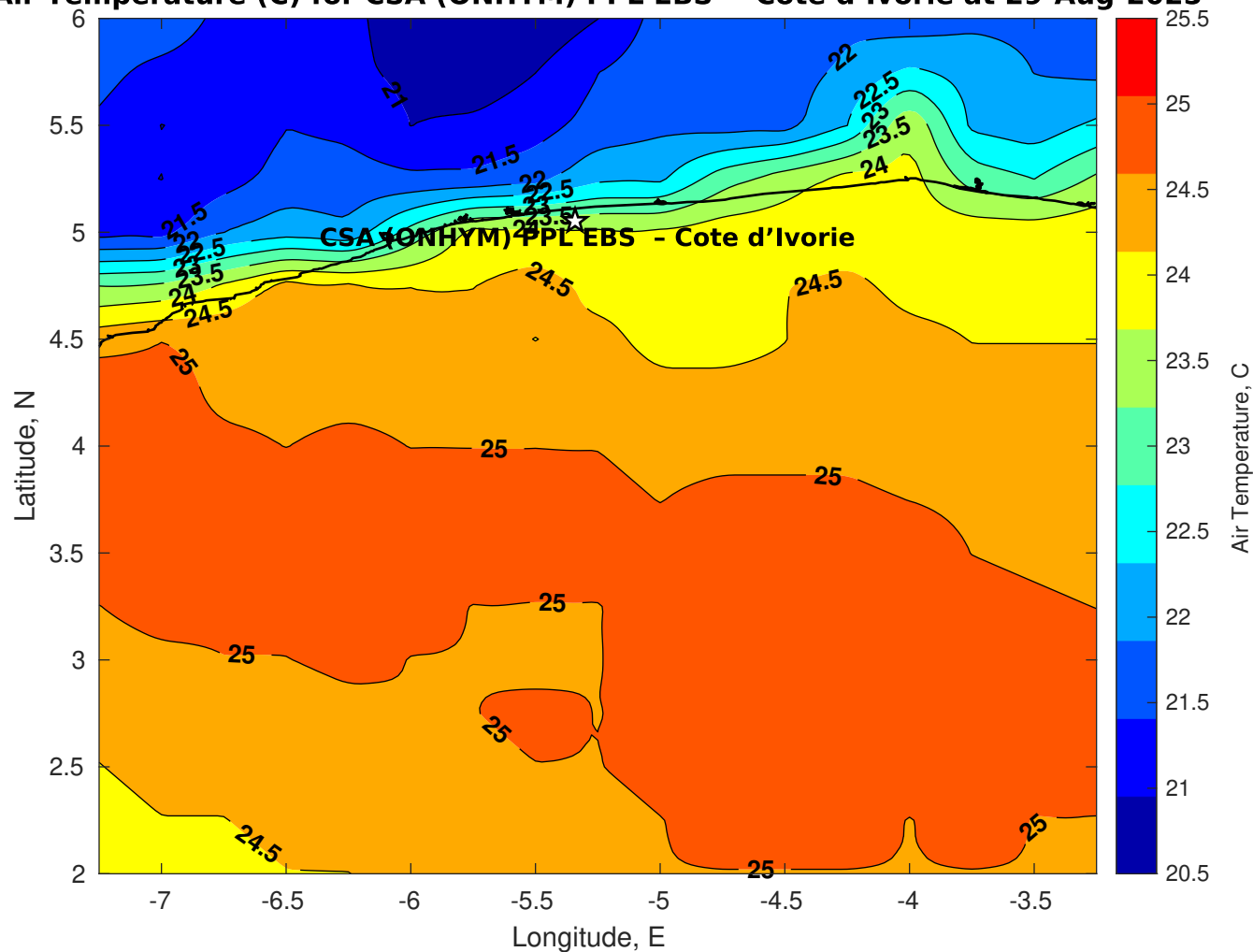
Air Temperature (C) for CSA (ONHYM) PPL EBS - Cote d'Ivoire at 29-Aug-2025
