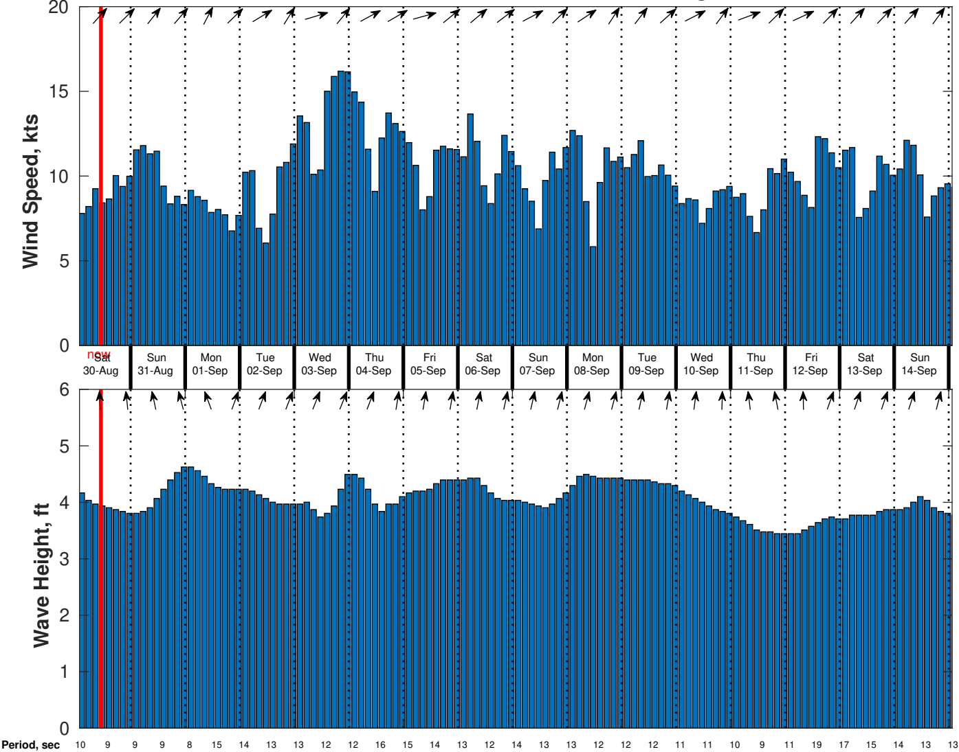
Wind & Wave Forecast for CSA (ONHYM) PPL EBS - Cote d'Ivoire from 29-Aug-2025 01:00:00 to 14-Sep-2025 01:00:00
