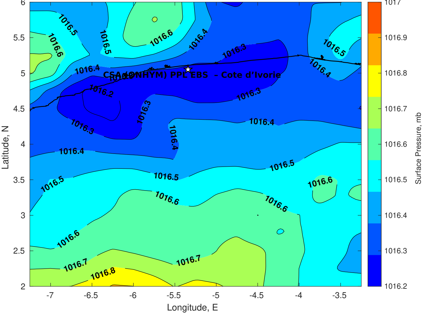
Surface Pressure (mb) for CSA (ONHYM) PPL EBS - Cote d'Ivoire at 31-Aug-2025 00:00:00
