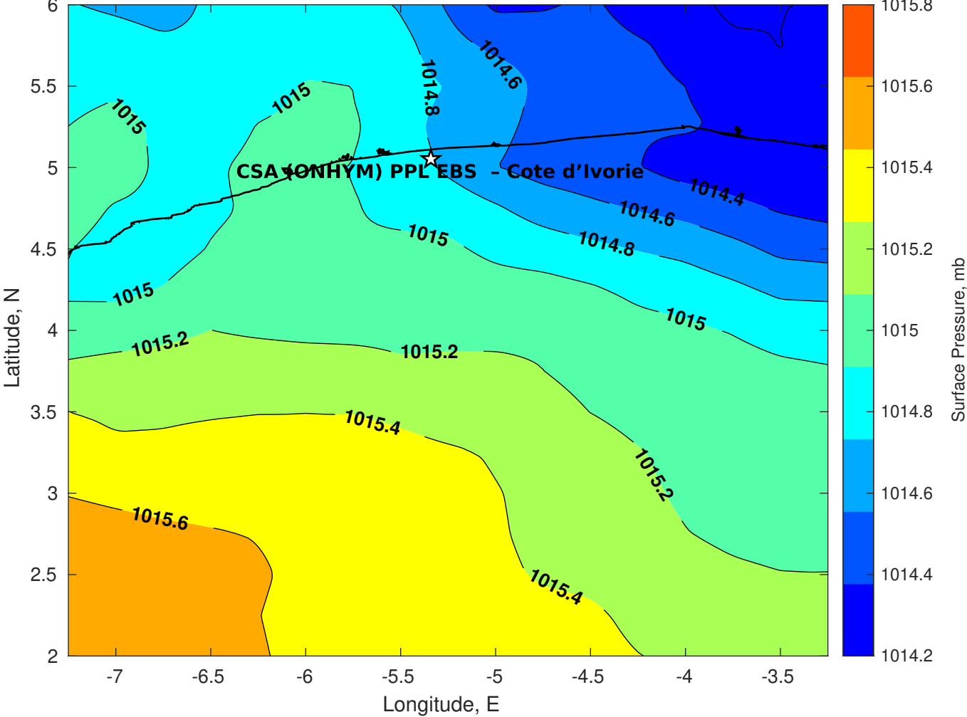
Surface Pressure (mb) for CSA (ONHYM) PPL EBS - Cote d'Ivoire at 30-Aug-2025 00:00:00
