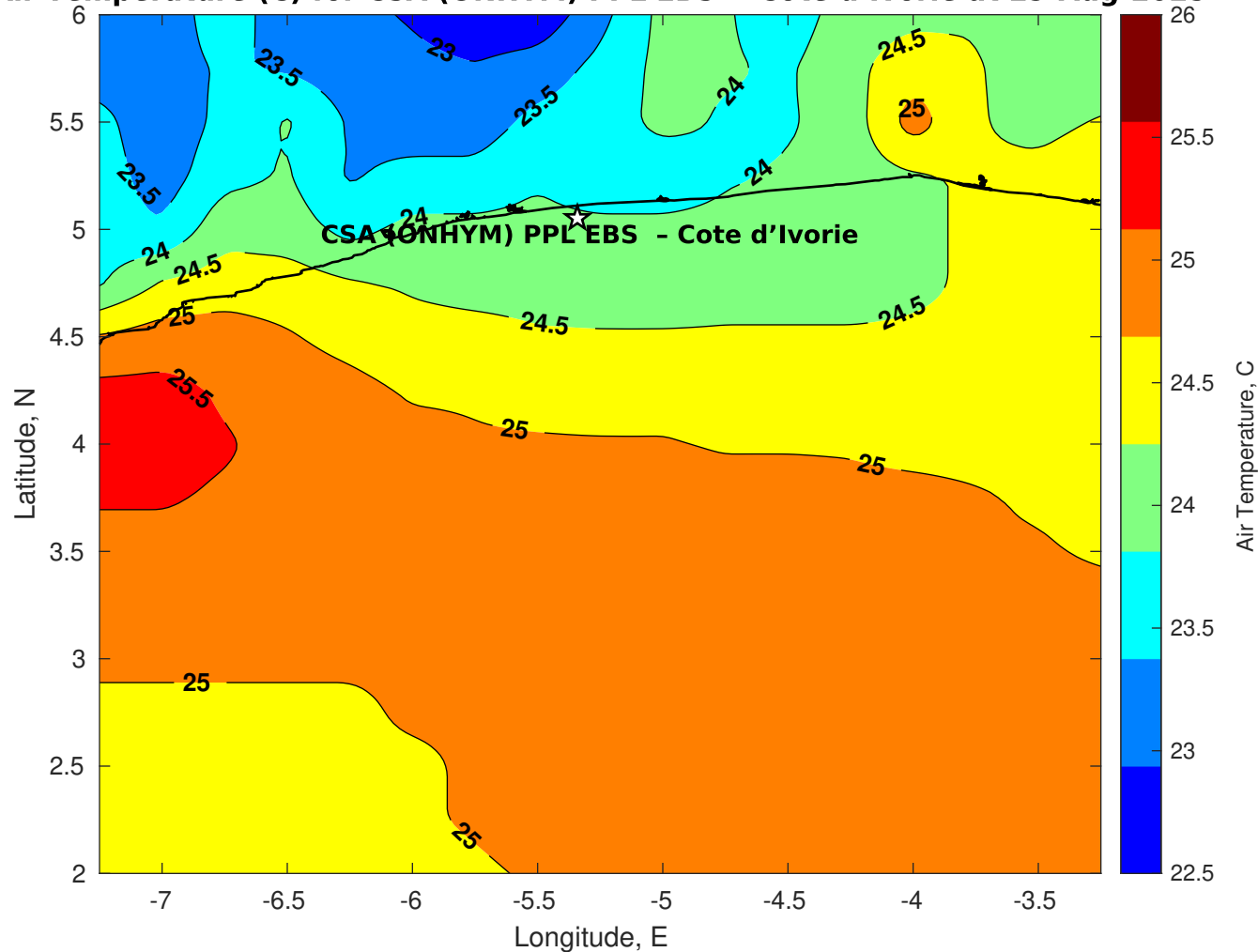
Air Temperature (C) for CSA (ONHYM) PPL EBS - Cote d'Ivoire at 29-Aug-2025
