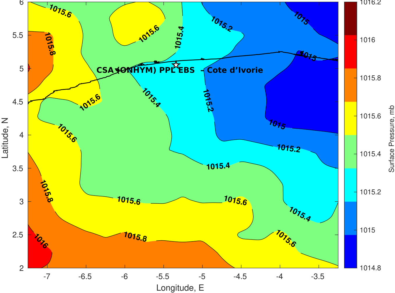
Surface Pressure (mb) for CSA (ONHYM) PPL EBS - Cote d'Ivoire at 29-Aug-2025 00:00:00
