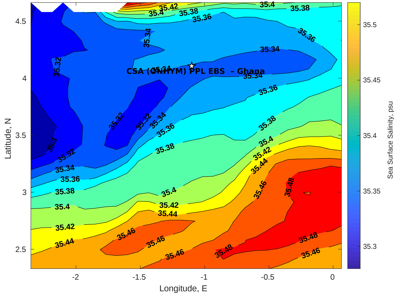
Surface Salinity for CSA (ONHYM) PPL EBS - Ghana at 28-Aug-2025 00:00:00
