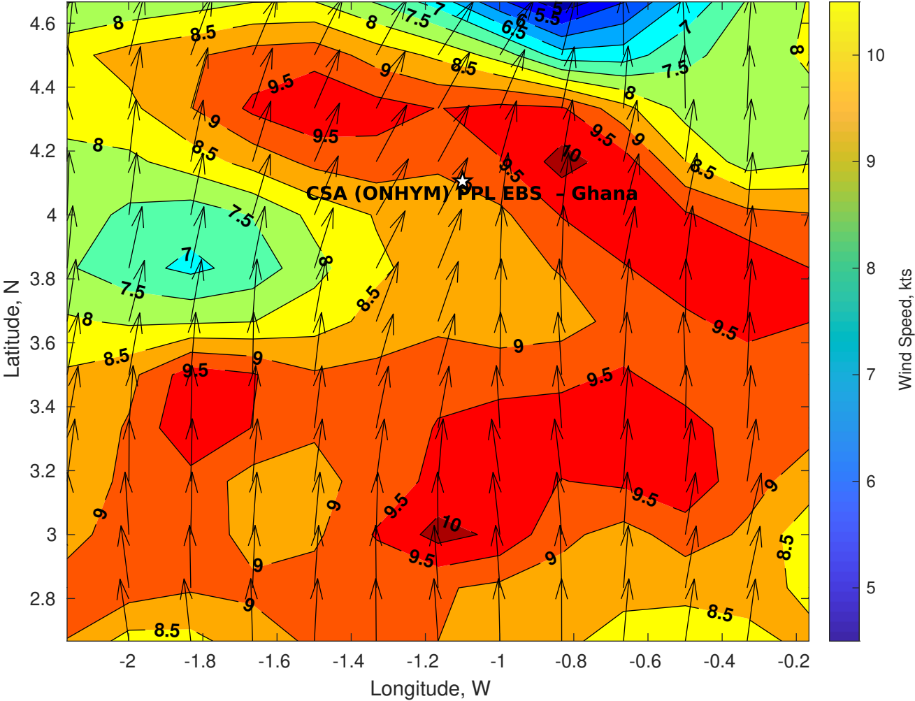
Winds (kts) for CSA (ONHYM) PPL EBS - Ghana at 29-Aug-2025 09:00:00
