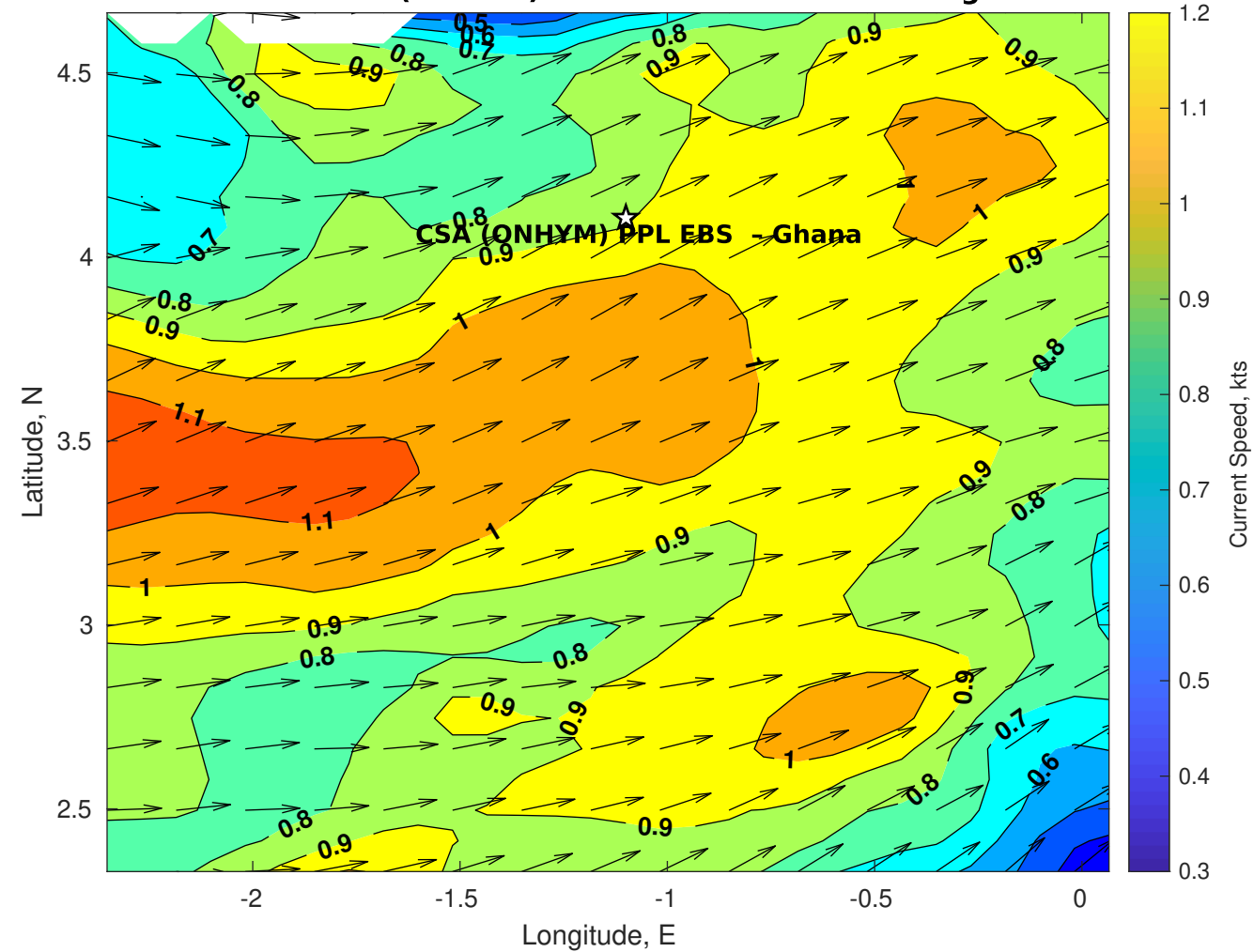
Surface Currents for CSA (ONHYM) PPL EBS - Ghana at 28-Aug-2025 00:00:00
