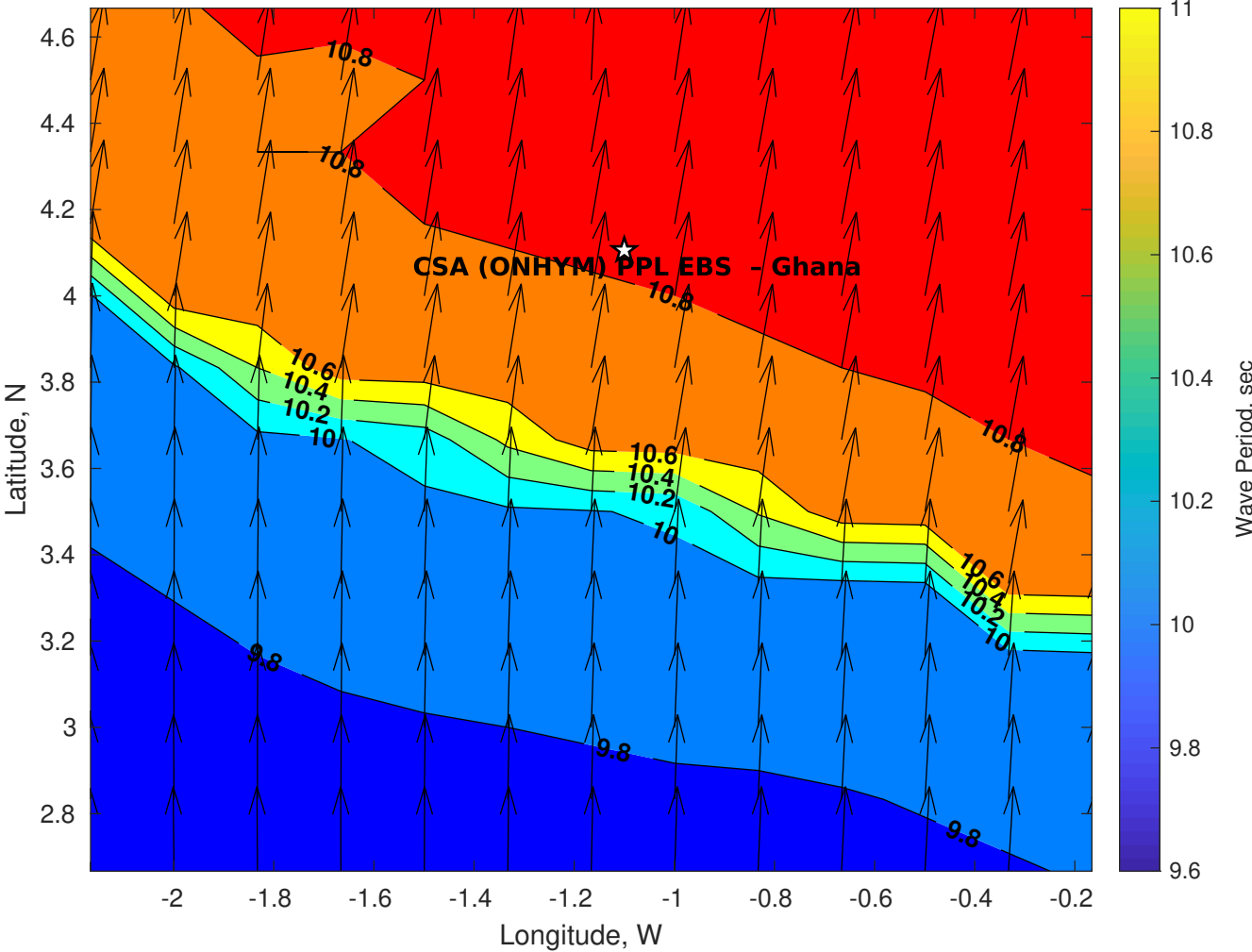
Wave Period (sec) for CSA (ONHYM) PPL EBS - Ghana at 29-Aug-2025 09:00:00
