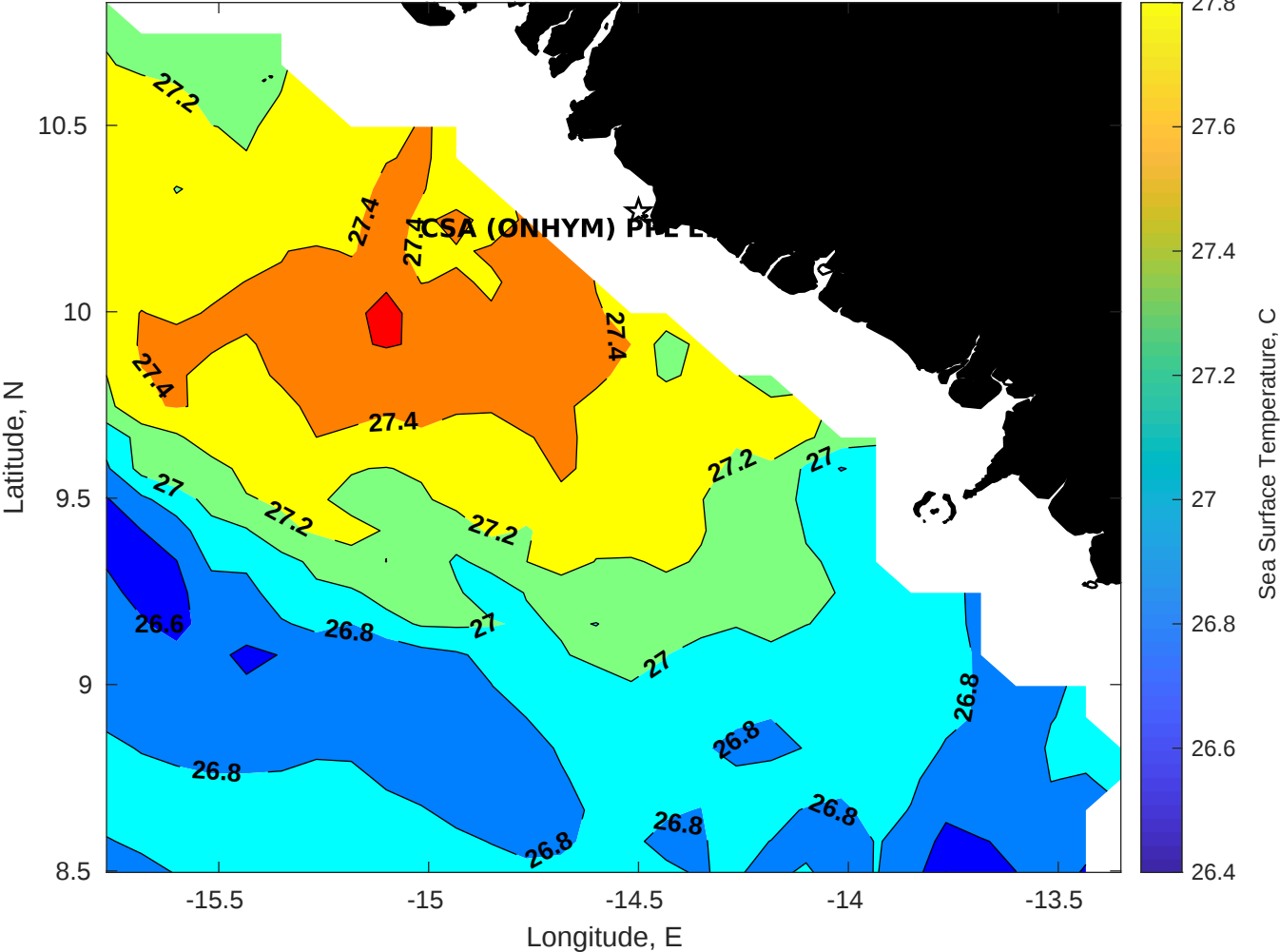
SST for CSA (ONHYM) PPL EBS - Guinea at 28-Aug-2025 00:00:00
