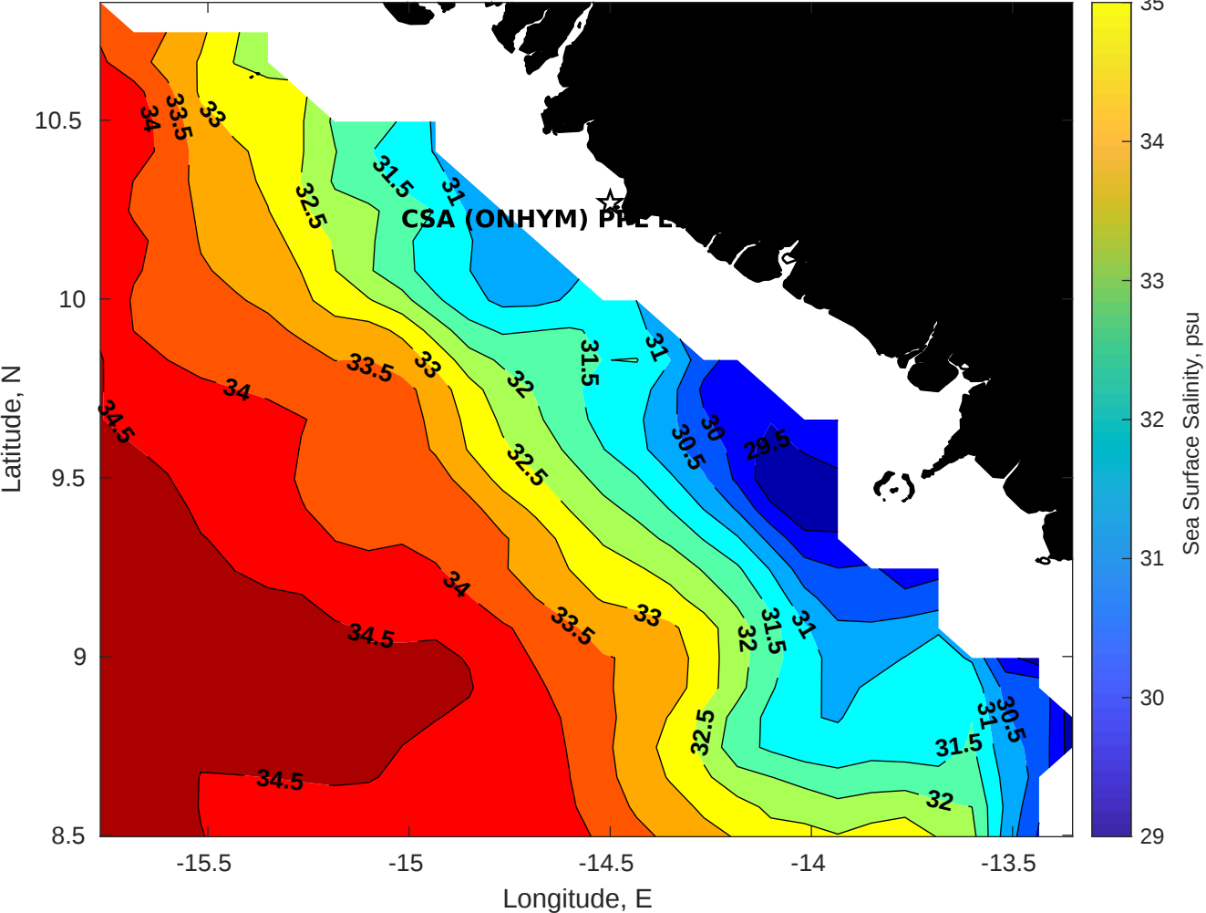
Surface Salinity for CSA (ONHYM) PPL EBS - Guinea at 28-Aug-2025 00:00:00
