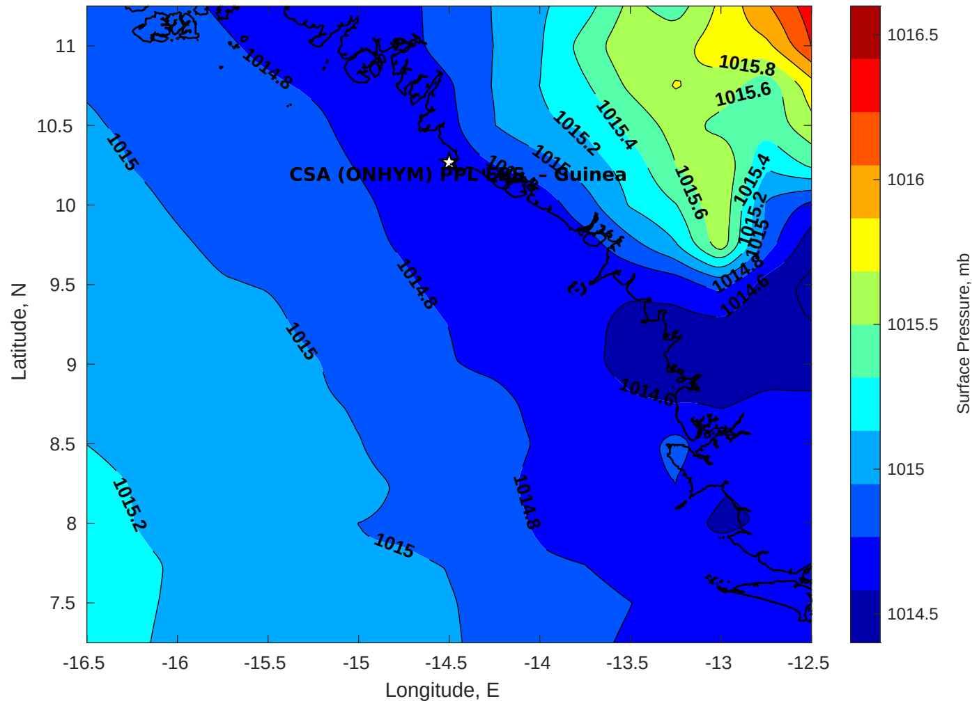
Surface Pressure (mb) for CSA (ONHYM) PPL EBS - Guinea at 30-Aug-2025 00:00:00
