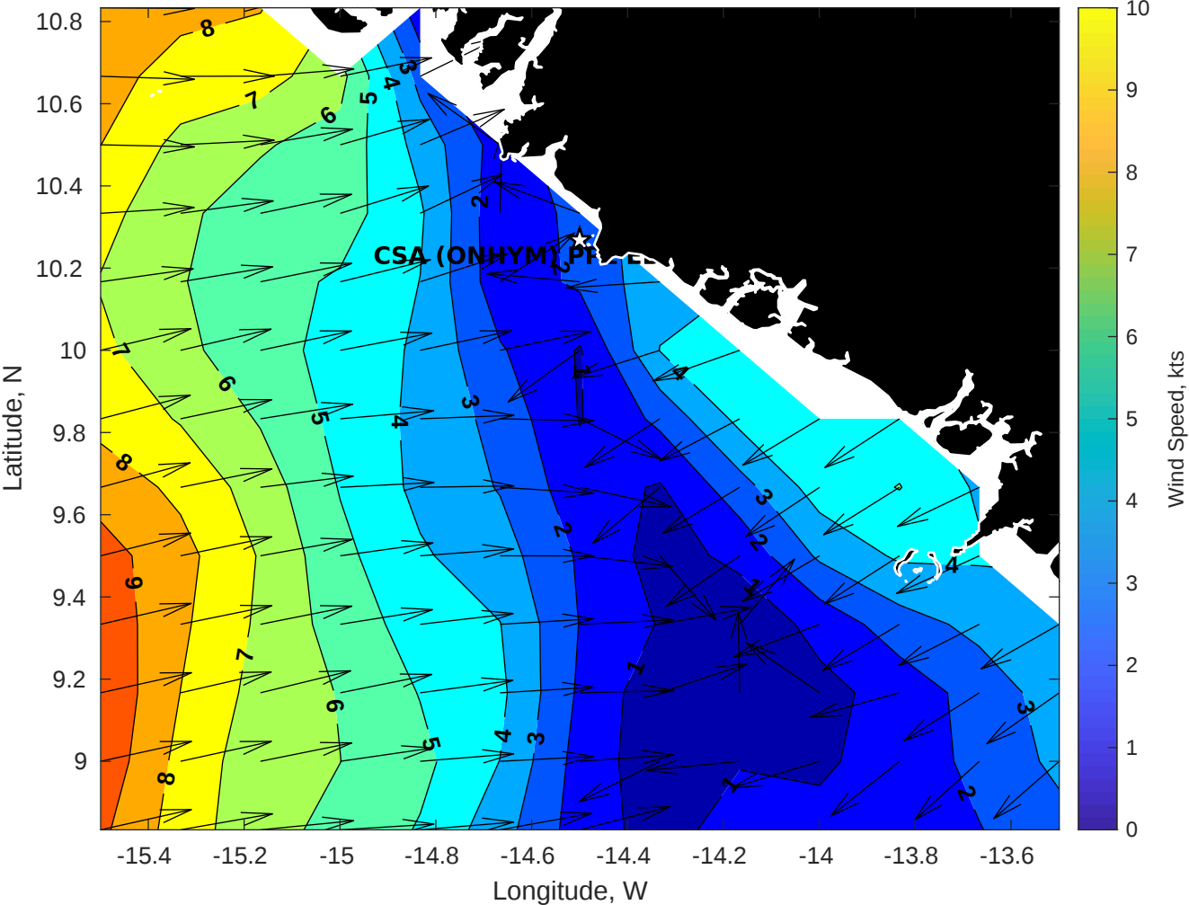
Winds (kts) for CSA (ONHYM) PPL EBS - Guinea at 29-Aug-2025 09:00:00
