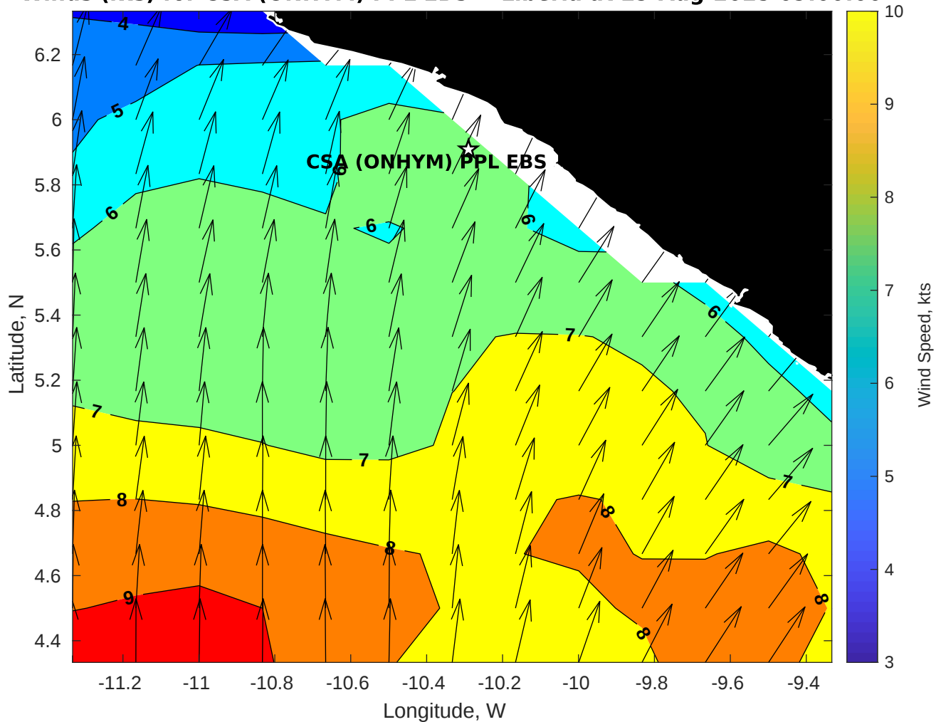
Winds (kts) for CSA (ONHYM) PPL EBS - Liberia at 29-Aug-2025 09:00:00
