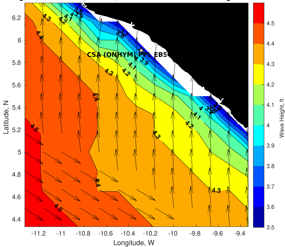
Wave Height (ft) for CSA (ONHYM) PPL EBS - Liberia at 29-Aug-2025 09:00:00
