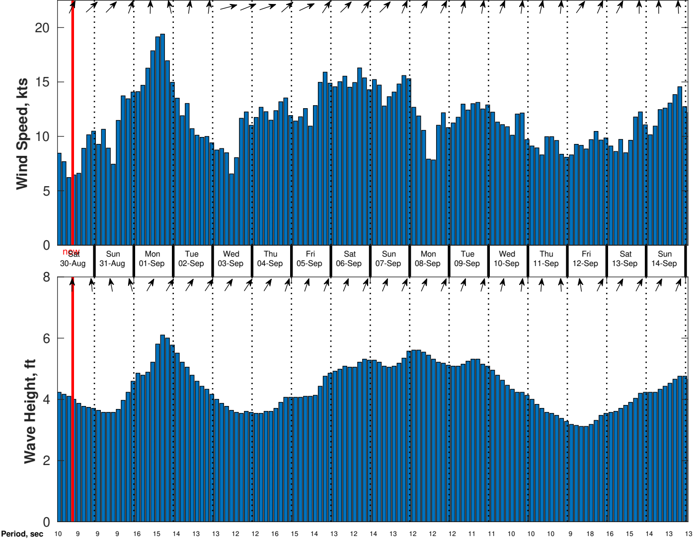
Wind & Wave Forecast for CSA (ONHYM) PPL EBS - Liberia from 29-Aug-2025 01:00:00 to 14-Sep-2025 01:00:00
