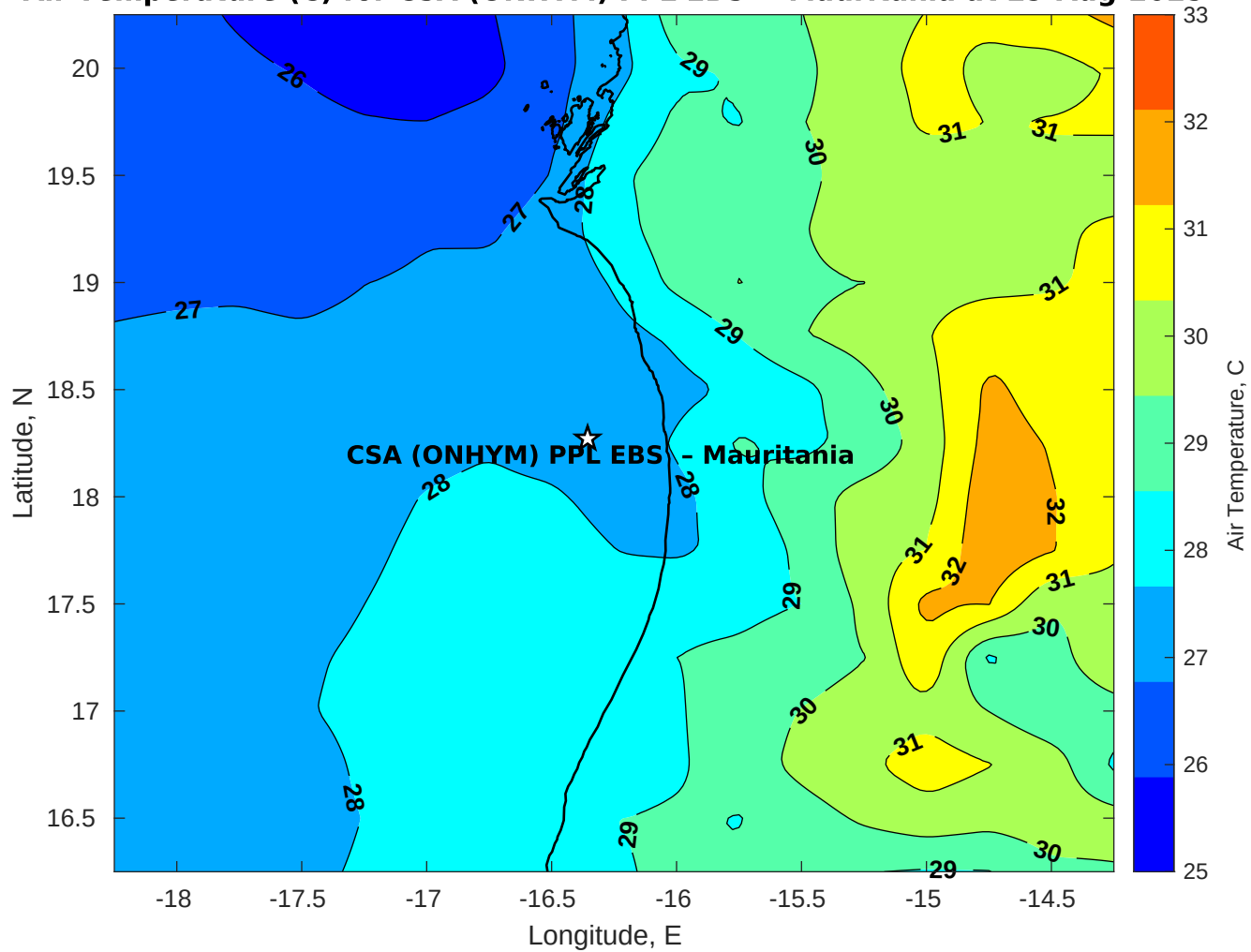
Air Temperature (C) for CSA (ONHYM) PPL EBS - Mauritania at 29-Aug-2025
