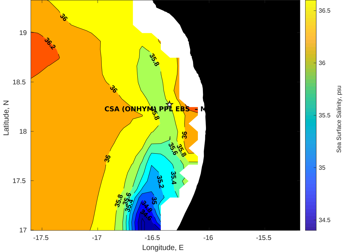
Surface Salinity for CSA (ONHYM) PPL EBS - Mauritania at 28-Aug-2025 00:00:00
