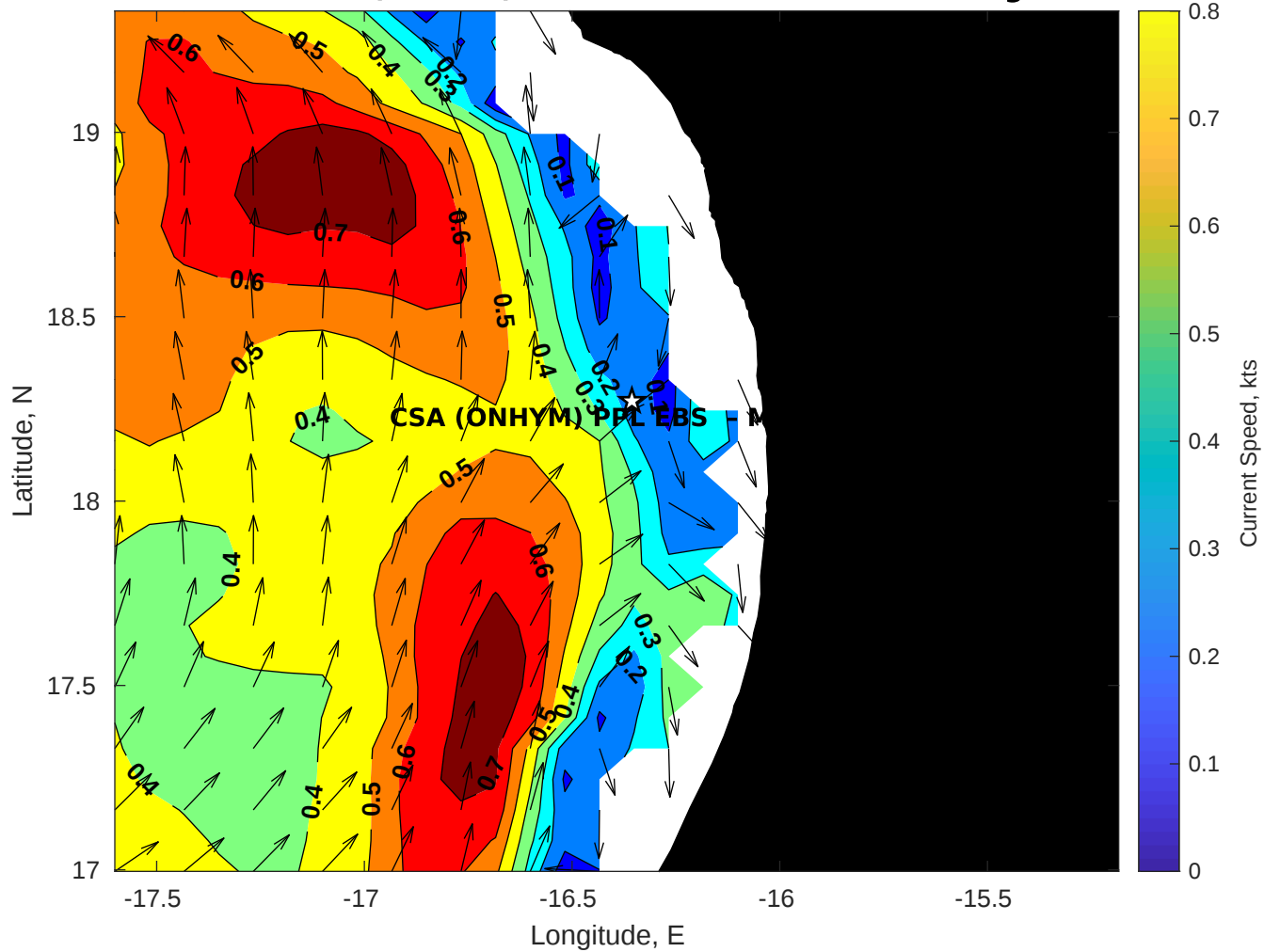
Surface Currents for CSA (ONHYM) PPL EBS - Mauritania at 28-Aug-2025 00:00:00
