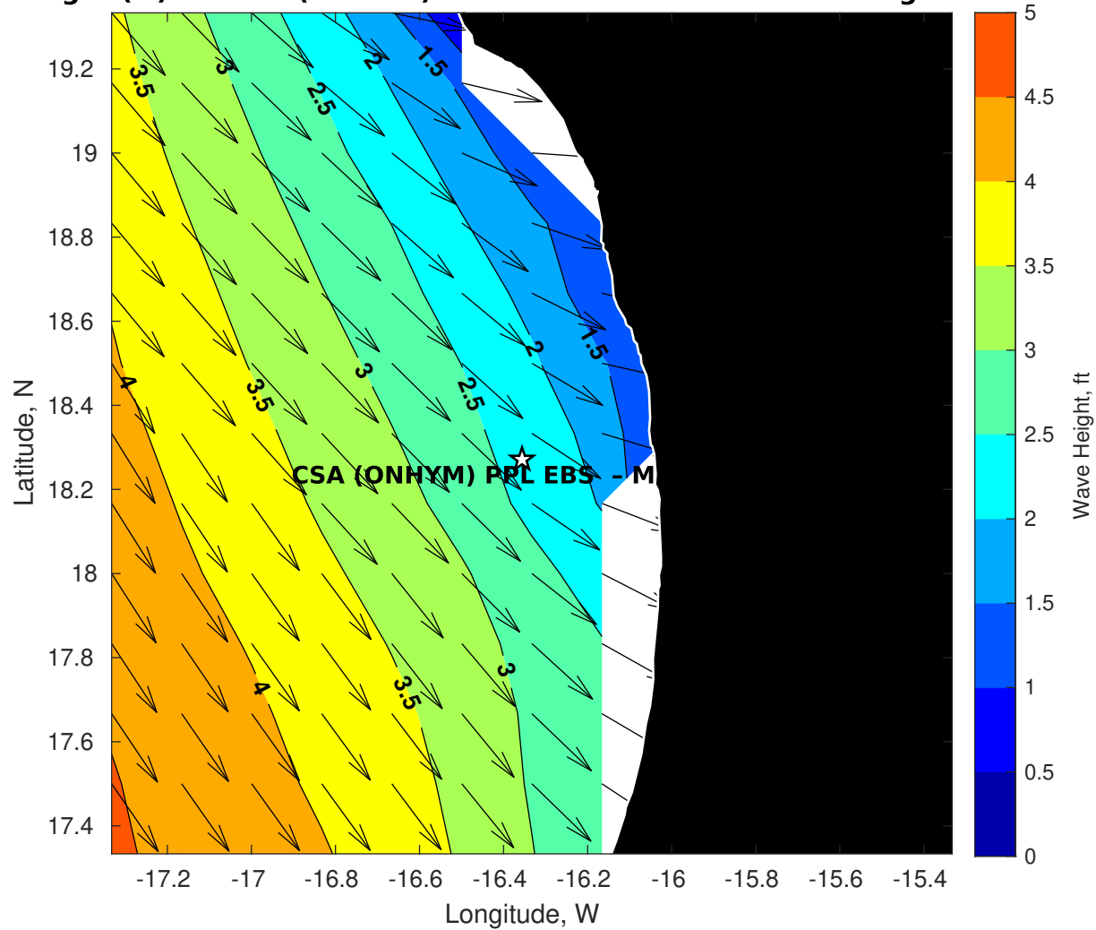
Wave Height (ft) for CSA (ONHYM) PPL EBS - Mauritania at 29-Aug-2025 09:00:00
