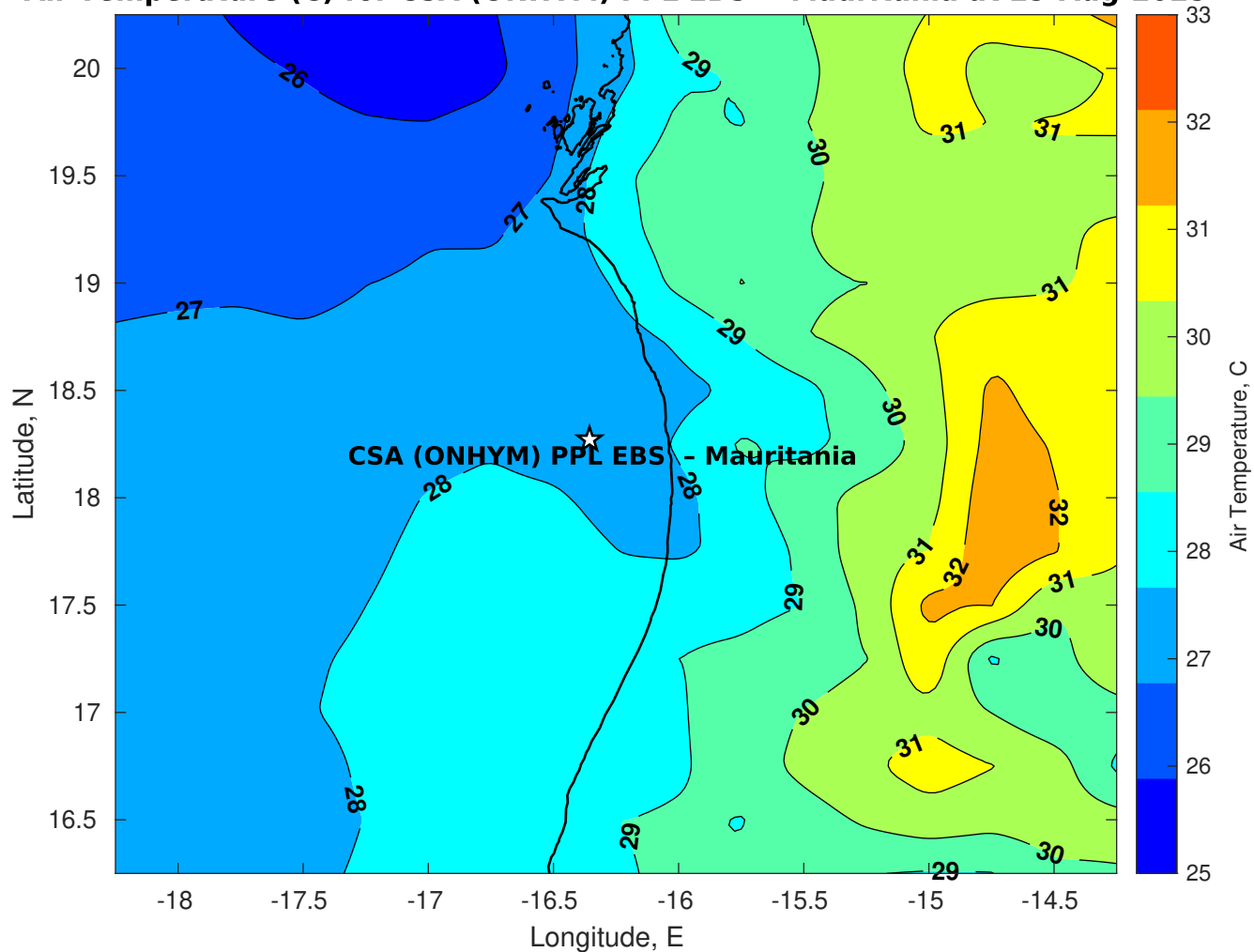
Air Temperature (C) for CSA (ONHYM) PPL EBS - Mauritania at 29-Aug-2025
