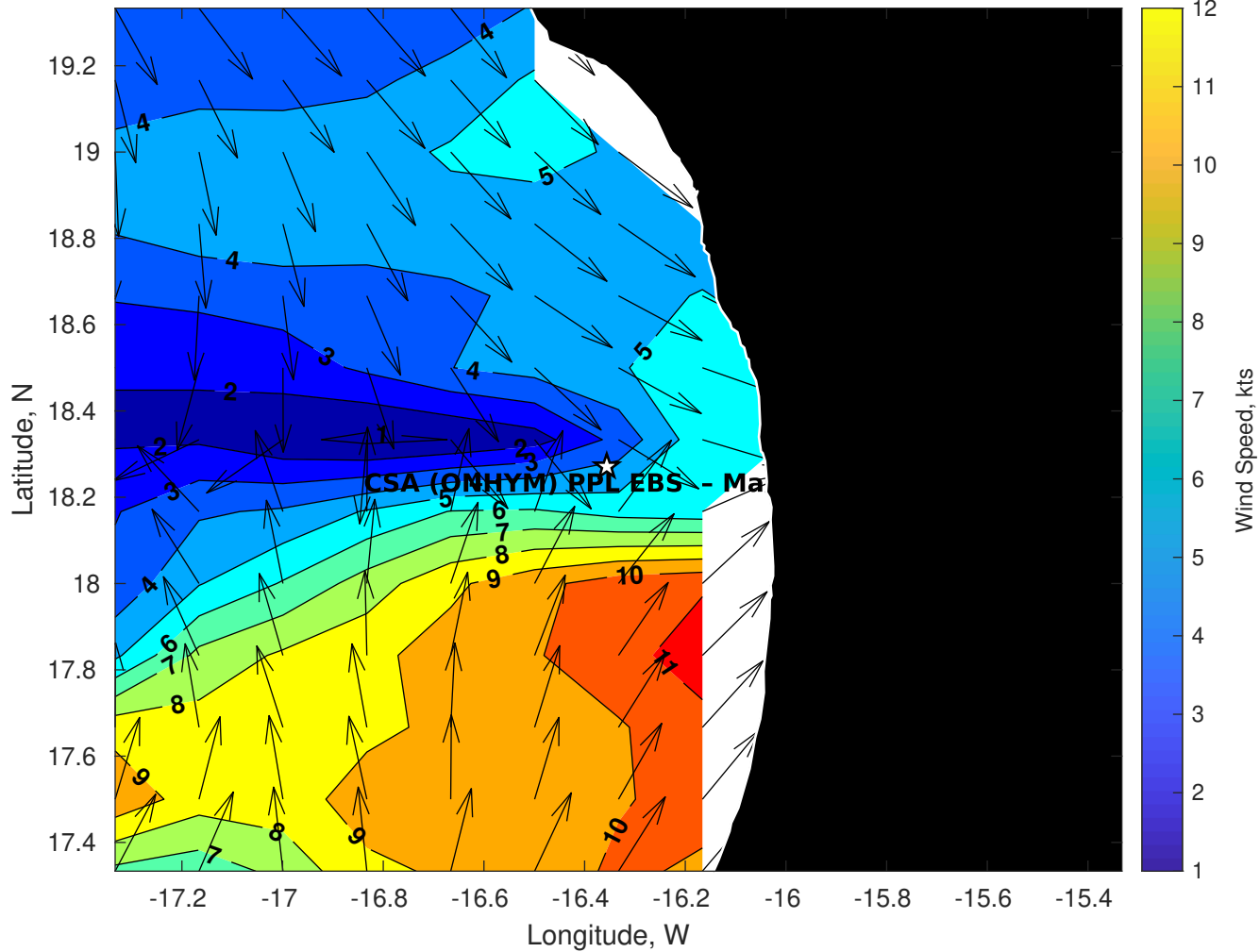
Winds (kts) for CSA (ONHYM) PPL EBS - Mauritania at 29-Aug-2025 09:00:00
