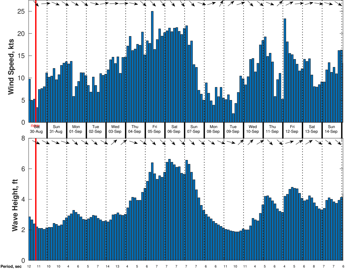
Wind & Wave Forecast for CSA (ONHYM) PPL EBS - Mauritania from 29-Aug-2025 01:00:00 to 14-Sep-2025 01:00:00
