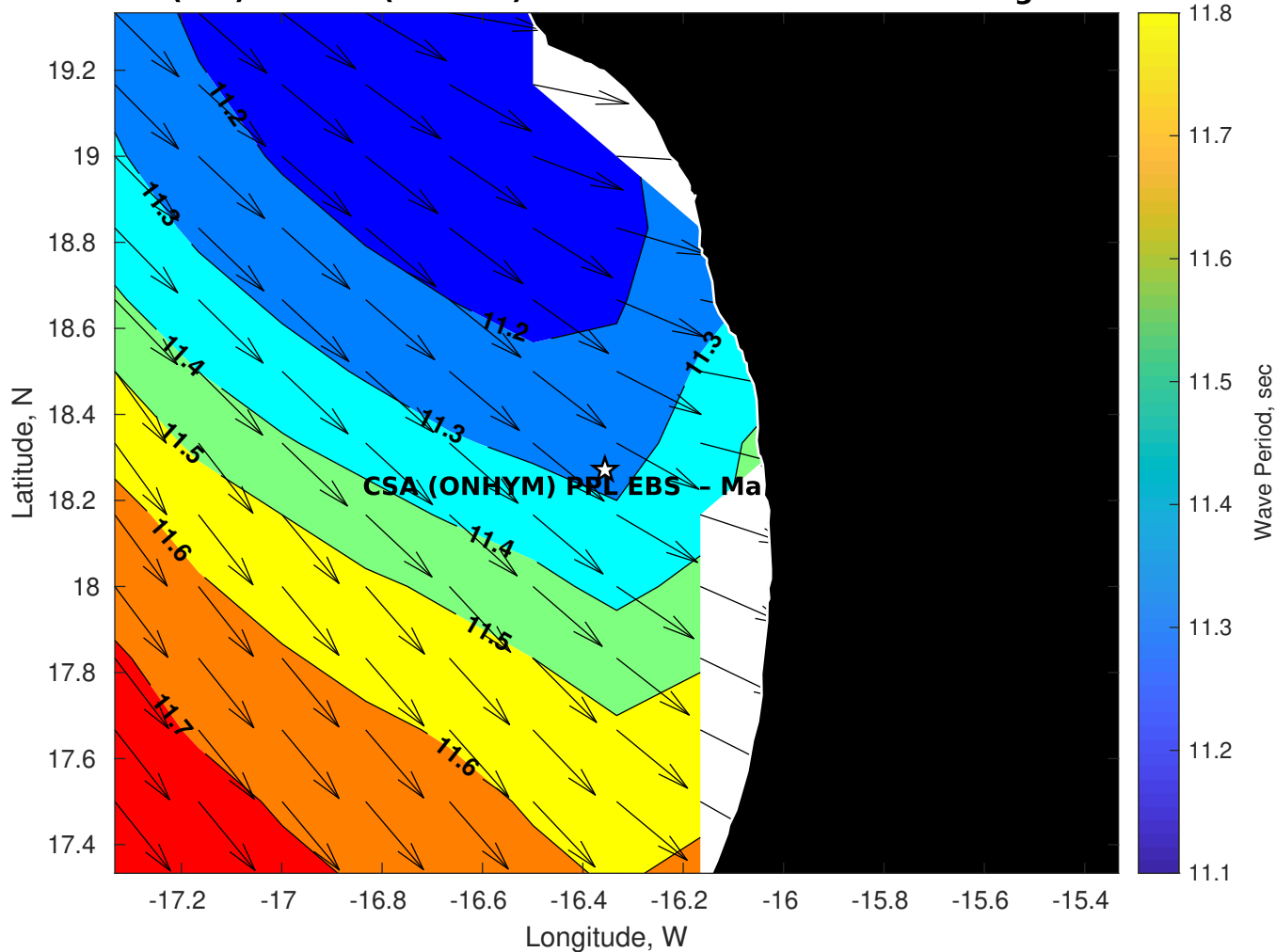
Wave Period (sec) for CSA (ONHYM) PPL EBS - Mauritania at 29-Aug-2025 09:00:00
