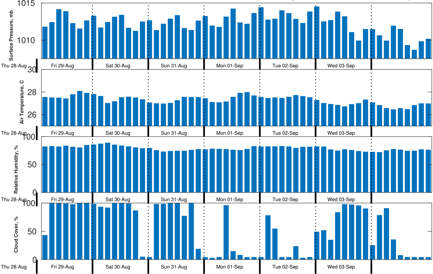
Met Forecast for CSA (ONHYM) PPL EBS - Mauritania from 29-Aug-2025 00:00:00 to 05-Sep-2025 00:00:00
