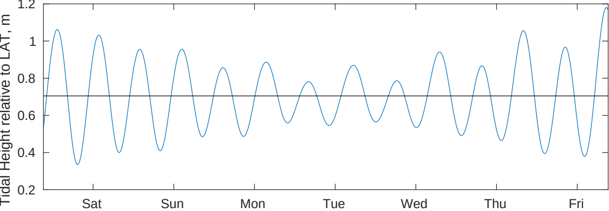
Tidal Currents and Heights for CSA (ONHYM) PPL EBS - Mauritania at 20250829
