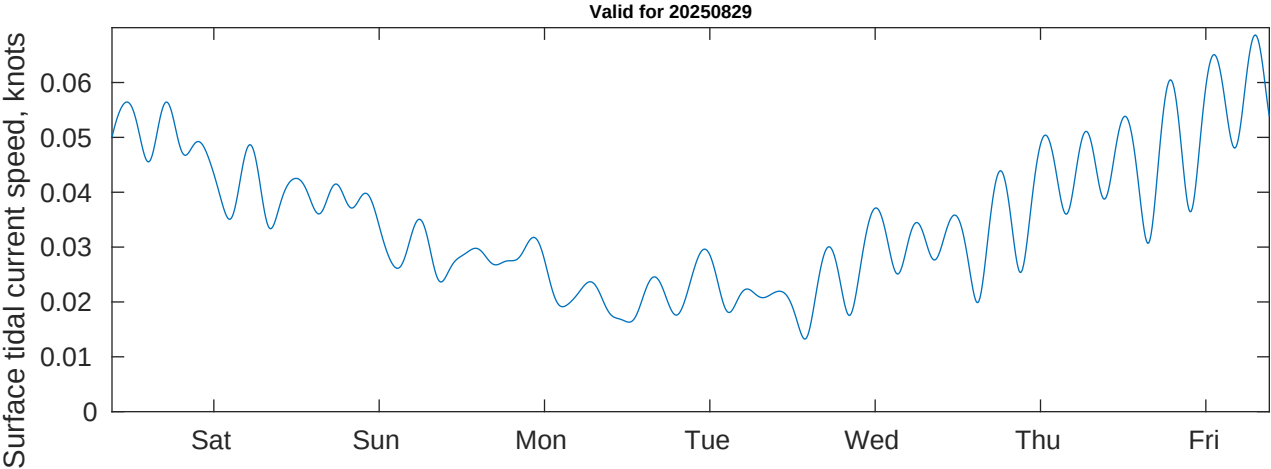
Tidal Currents and Heights for CSA (ONHYM) PPL EBS - Mauritania at 20250829
