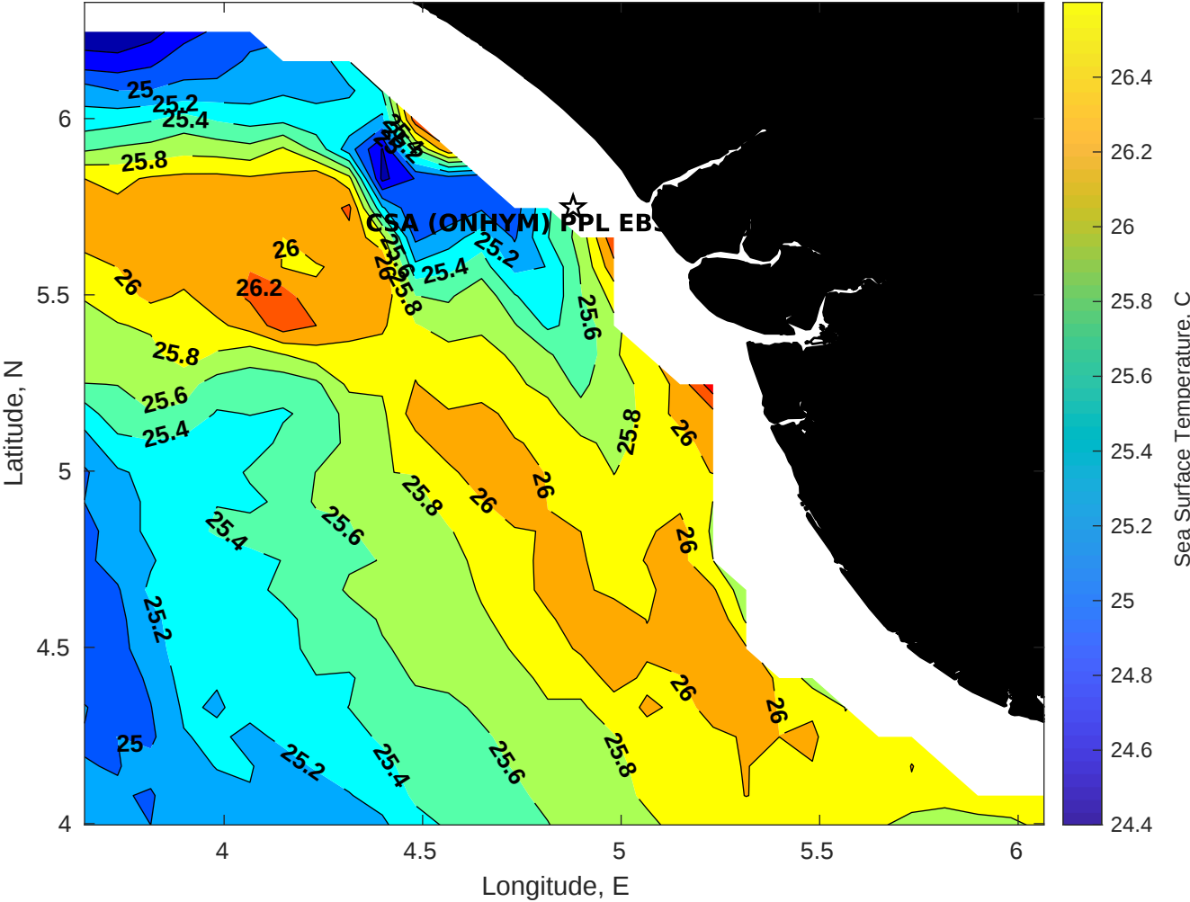
SST for CSA (ONHYM) PPL EBS - Nigeria at 28-Aug-2025 00:00:00
