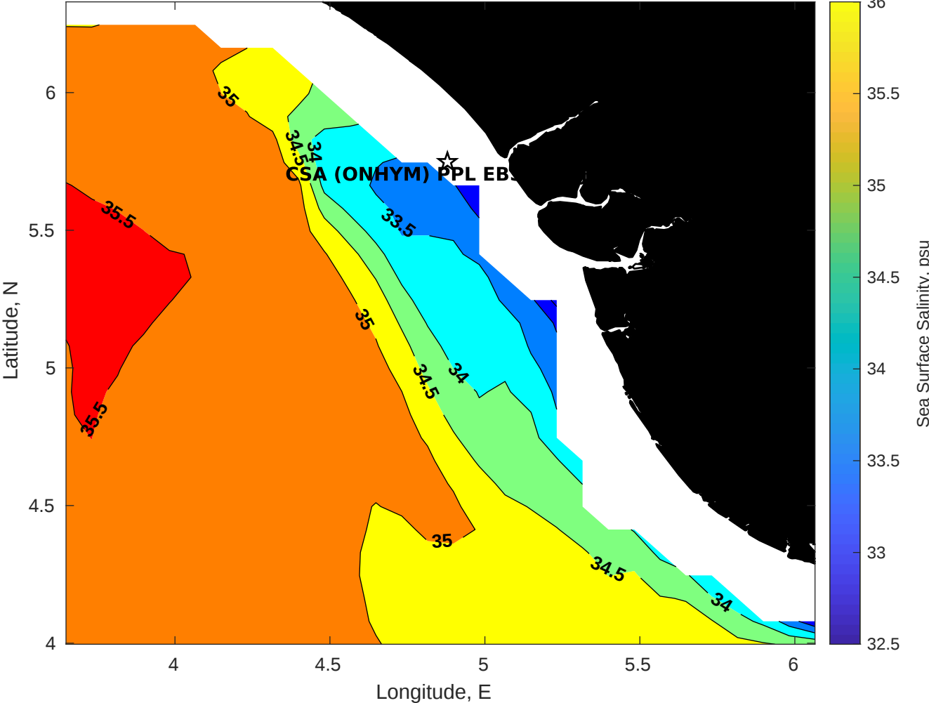
Surface Salinity for CSA (ONHYM) PPL EBS - Nigeria at 28-Aug-2025 00:00:00
