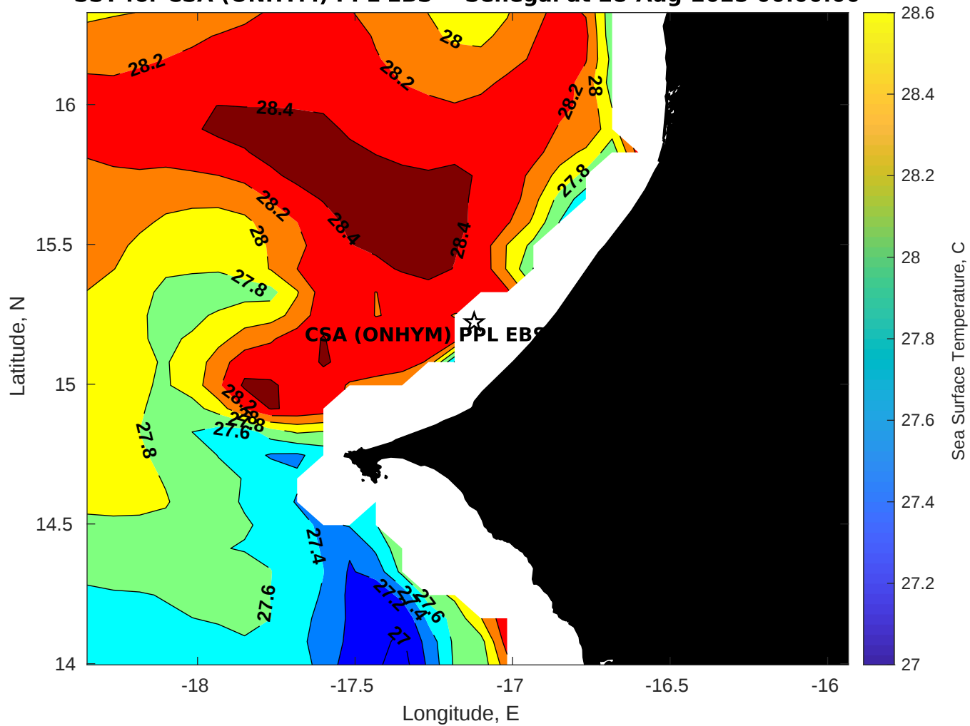
SST for CSA (ONHYM) PPL EBS - Senegal at 28-Aug-2025 00:00:00
