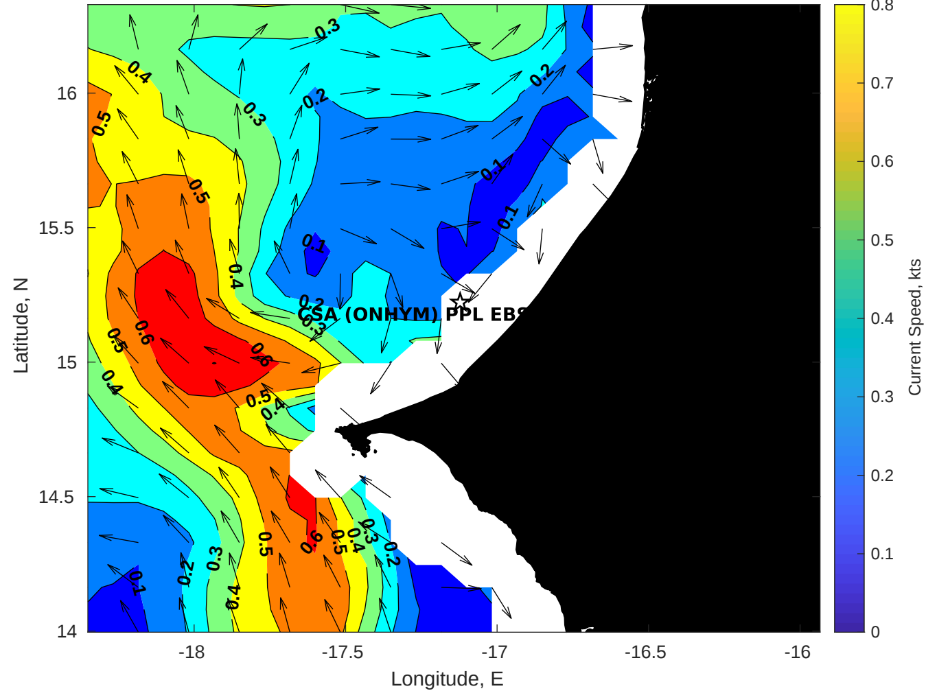
Surface Currents for CSA (ONHYM) PPL EBS - Senegal at 28-Aug-2025 00:00:00
