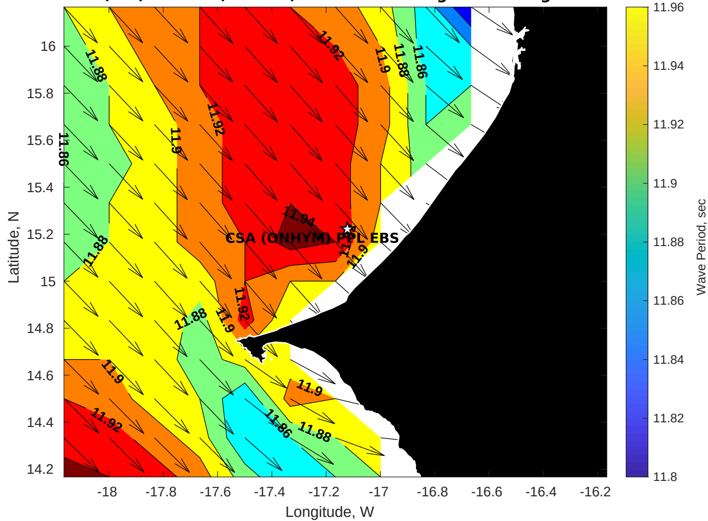
Wave Period (sec) for CSA (ONHYM) PPL EBS - Senegal at 29-Aug-2025 09:00:00
