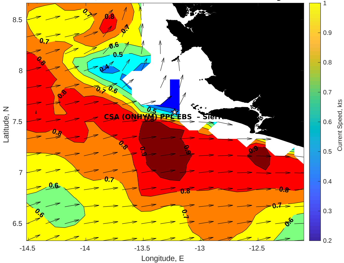
Surface Currents for CSA (ONHYM) PPL EBS - Sierra Leone at 28-Aug-2025 00:00:00
