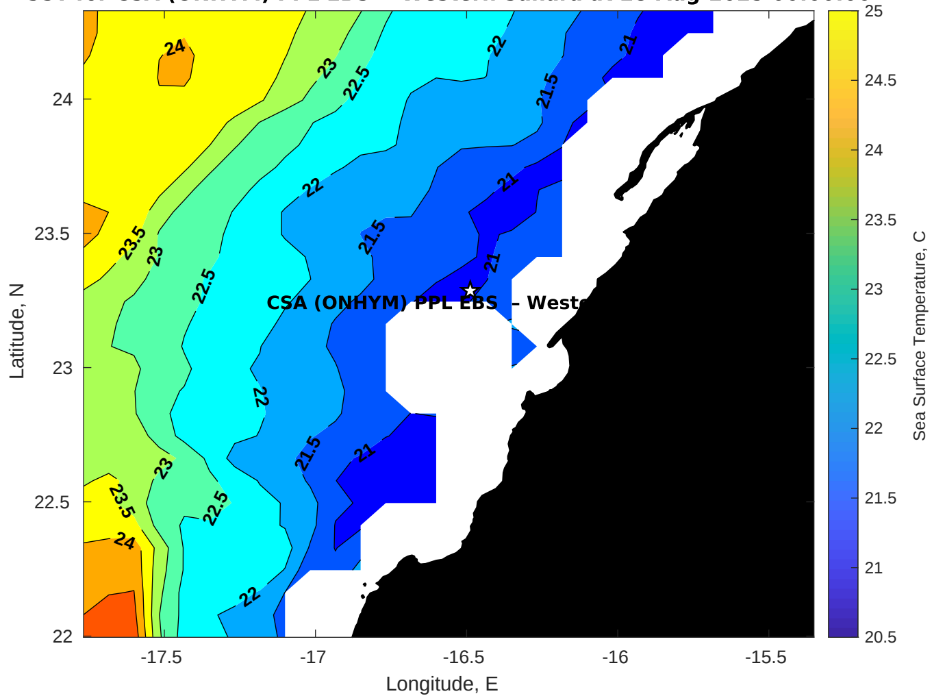
SST for CSA (ONHYM) PPL EBS - Western Sahara at 28-Aug-2025 00:00:00
