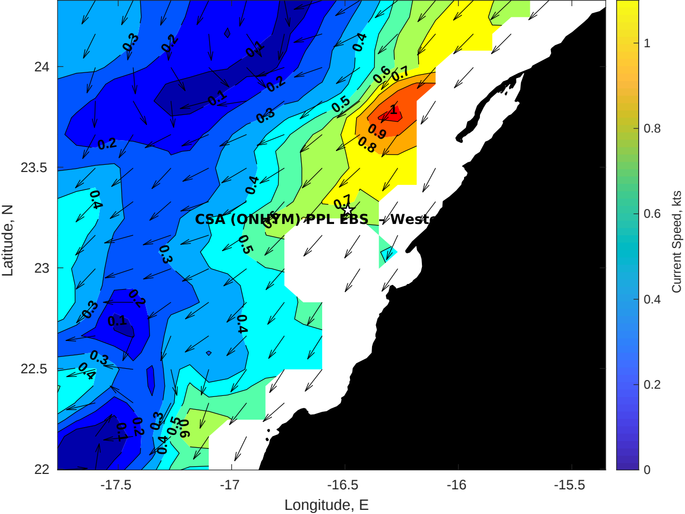
Surface Currents for CSA (ONHYM) PPL EBS - Western Sahara at 28-Aug-2025 00:00:00
