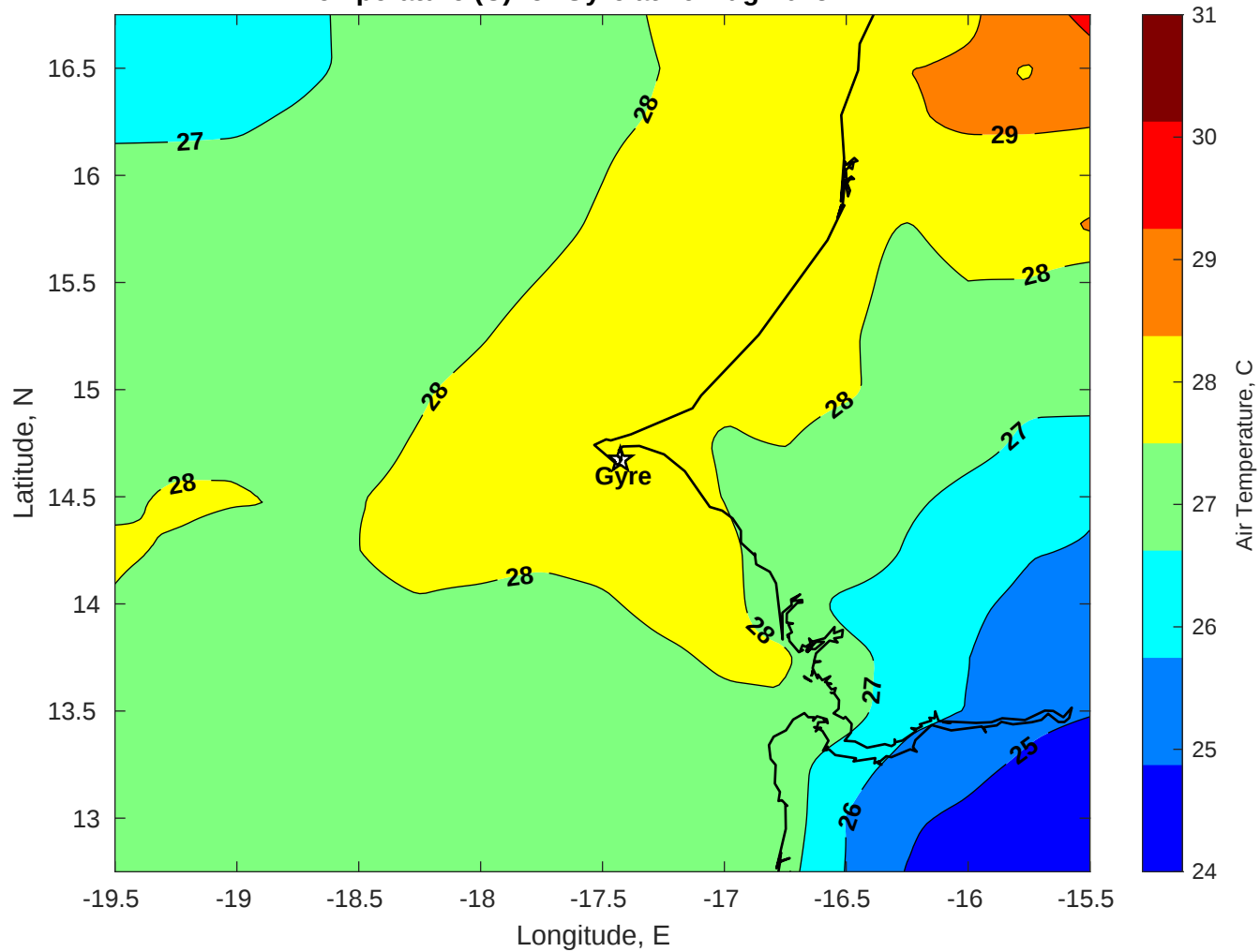
Air Temperature (C) for Gyre at 29-Aug-2025
