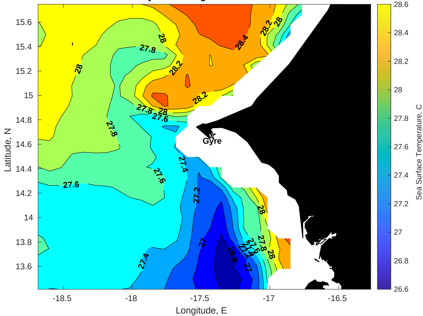
SST for Gyre at 28-Aug-2025 00:00:00
