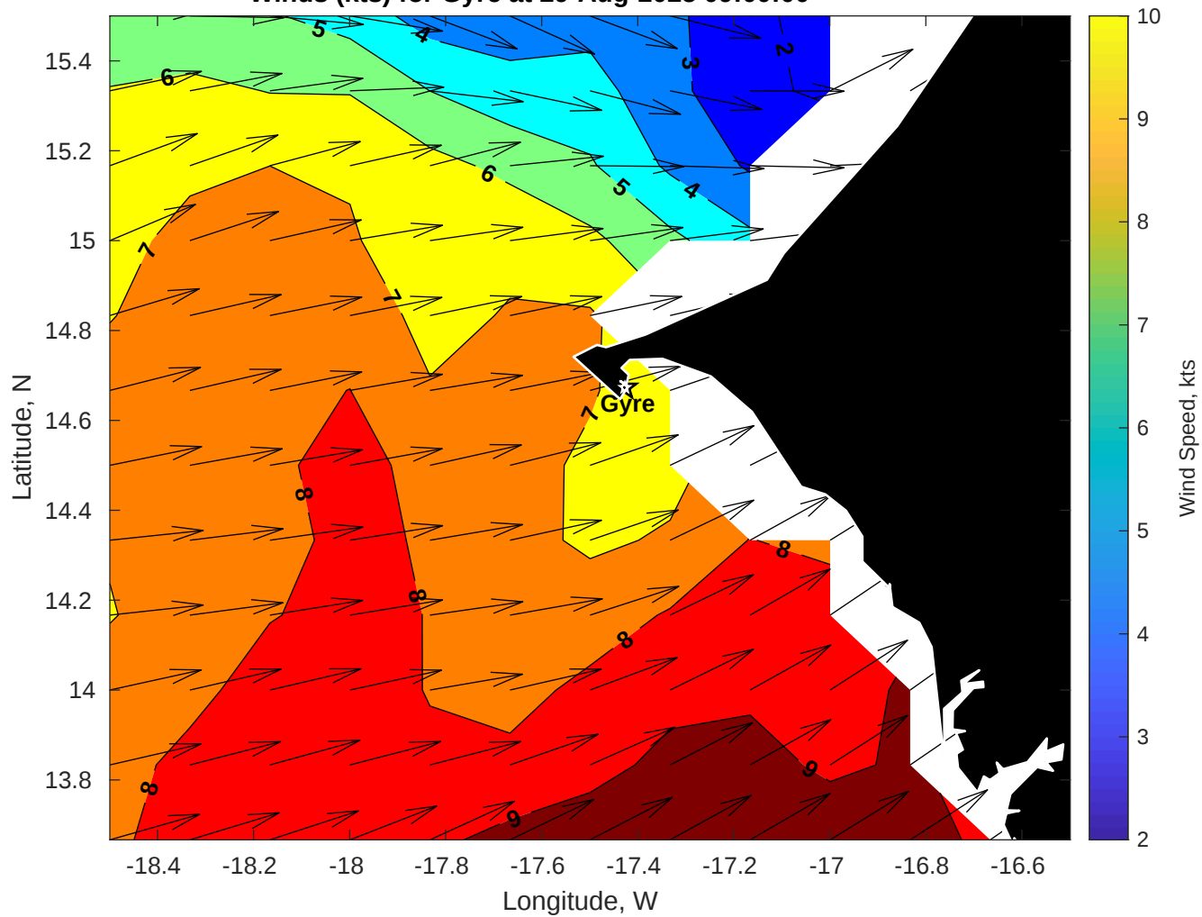
Winds (kts) for Gyre at 29-Aug-2025 09:00:00
