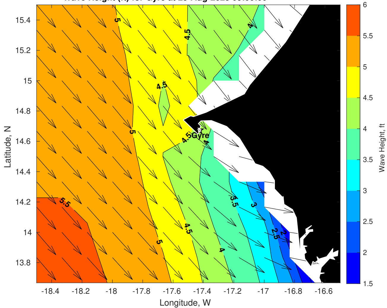
Wave Height (ft) for Gyre at 29-Aug-2025 09:00:00
