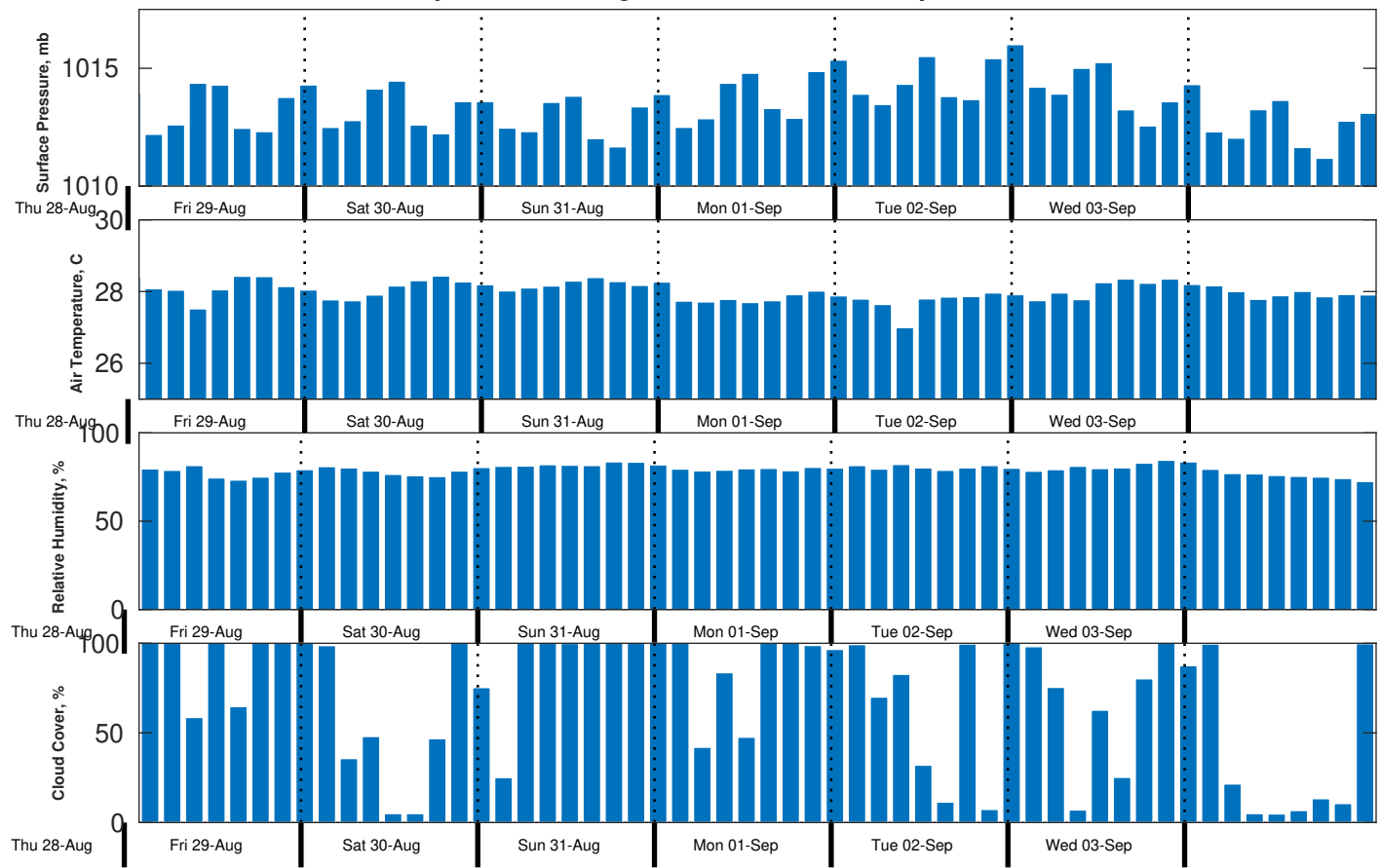
Met Forecast for Gyre from 28-Aug-2025 23:00:00 to 04-Sep-2025 23:00:00
