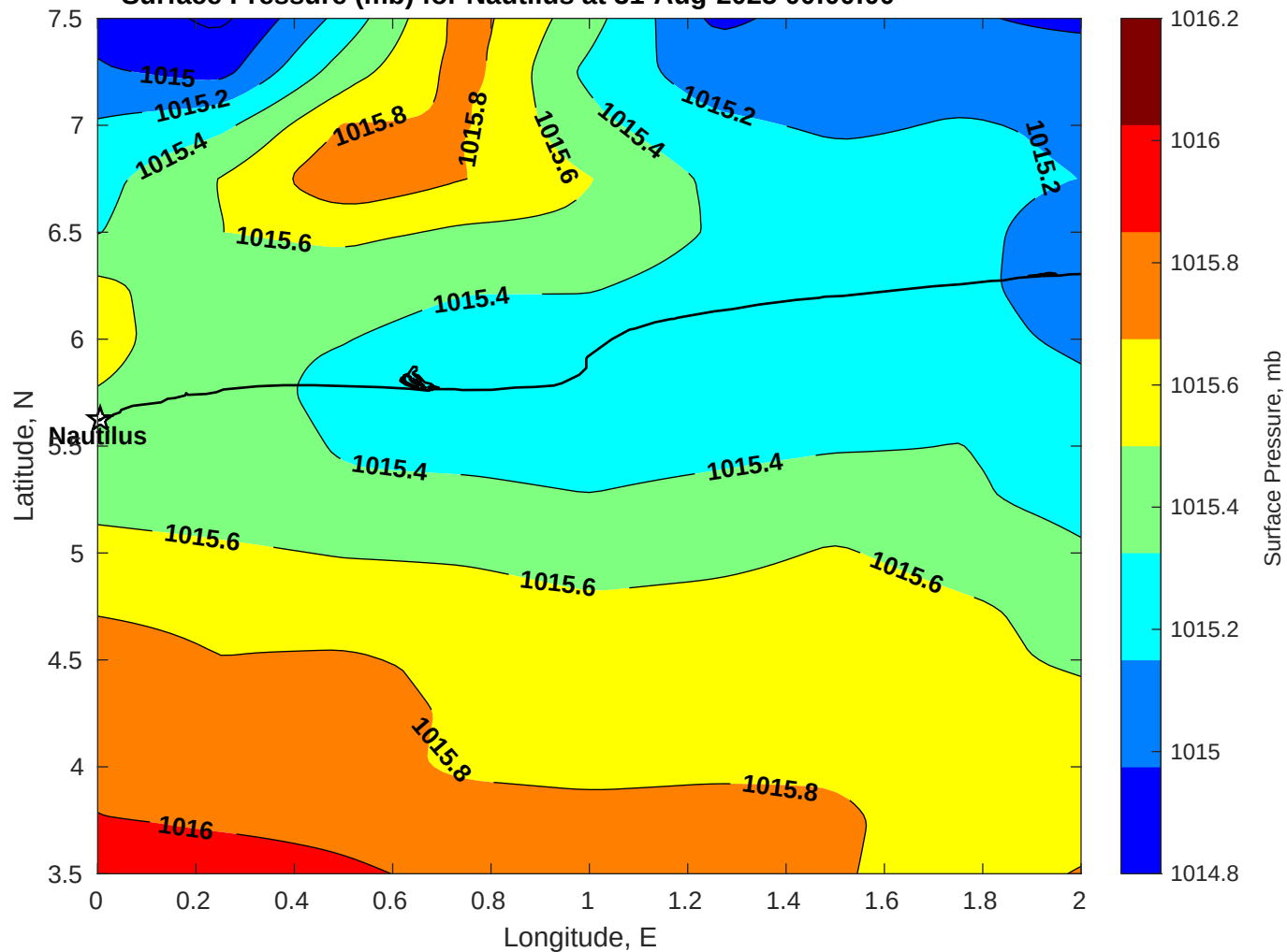
Surface Pressure (mb) for Nautilus at 31-Aug-2025 00:00:00
