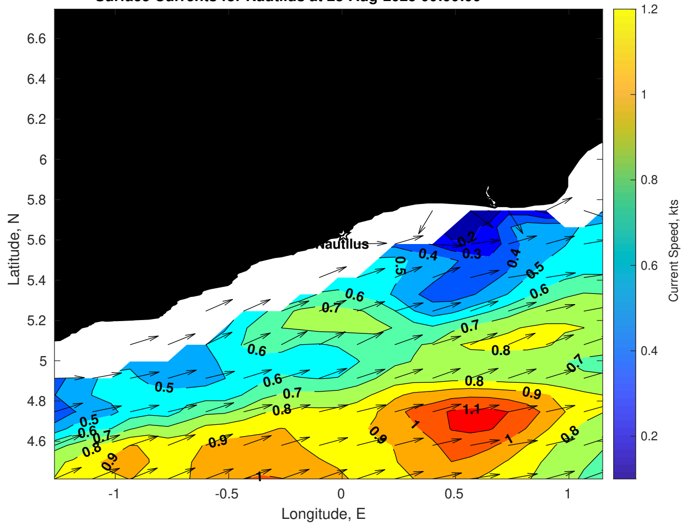
Surface Currents for Nautilus at 28-Aug-2025 00:00:00
