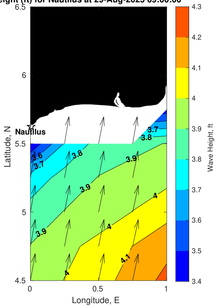
Wave Height (ft) for Nautilus at 29-Aug-2025 09:00:00
