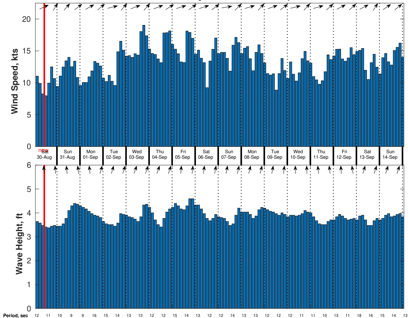
Wind & Wave Forecast for Nautilus from 29-Aug-2025 02:00:00 to 14-Sep-2025 02:00:00
