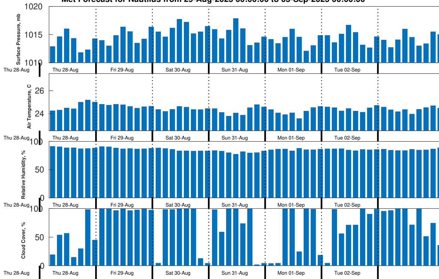
Met Forecast for Nautilus from 29-Aug-2025 00:00:00 to 05-Sep-2025 00:00:00
