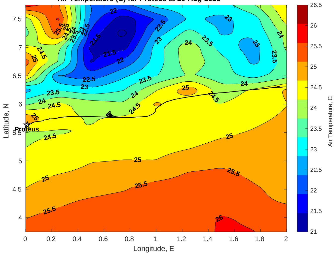
Air Temperature (C) for Proteus at 29-Aug-2025
