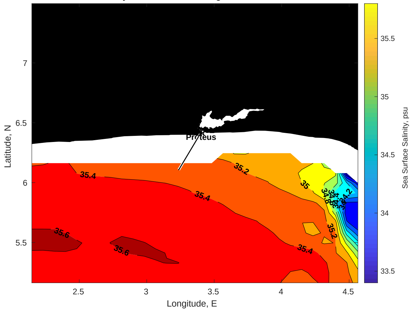
Surface Salinity for Proteus at 28-Aug-2025 00:00:00
