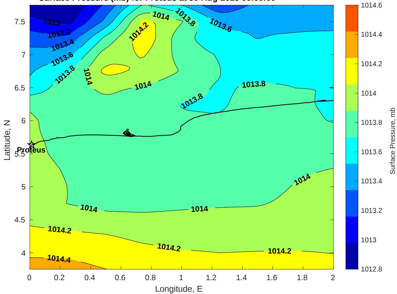
Surface Pressure (mb) for Proteus at 30-Aug-2025 00:00:00
