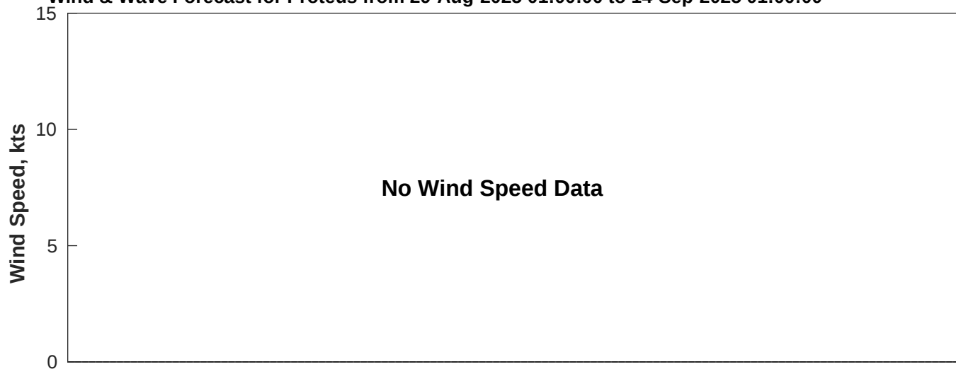
Wind & Wave Forecast for Proteus from 29-Aug-2025 01:00:00 to 14-Sep-2025 01:00:00
