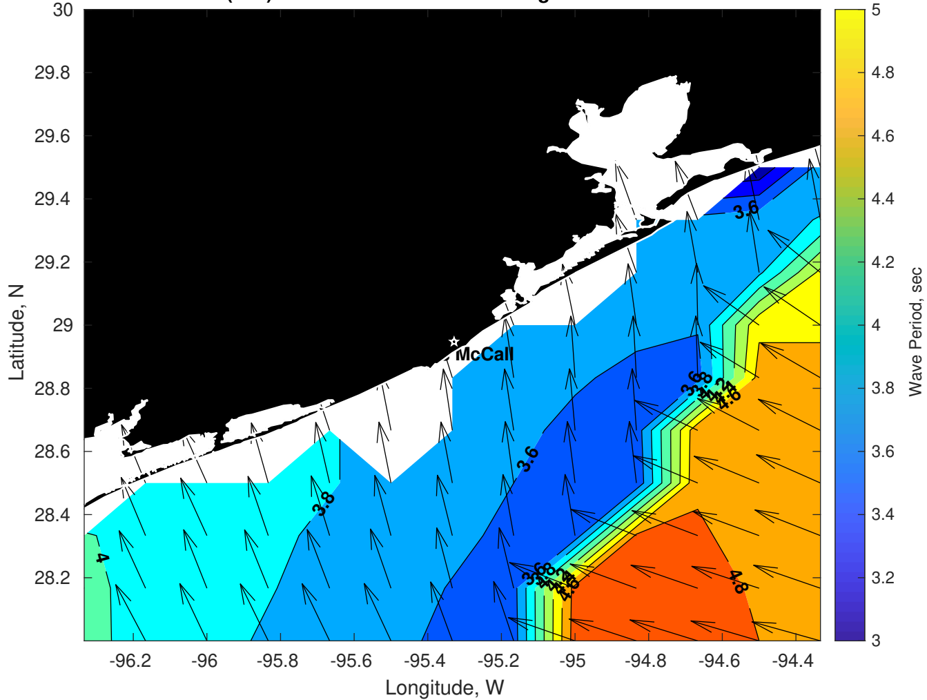
Wave Period (sec) for Brooks McCall at 30-Aug-2025 09:00:00
