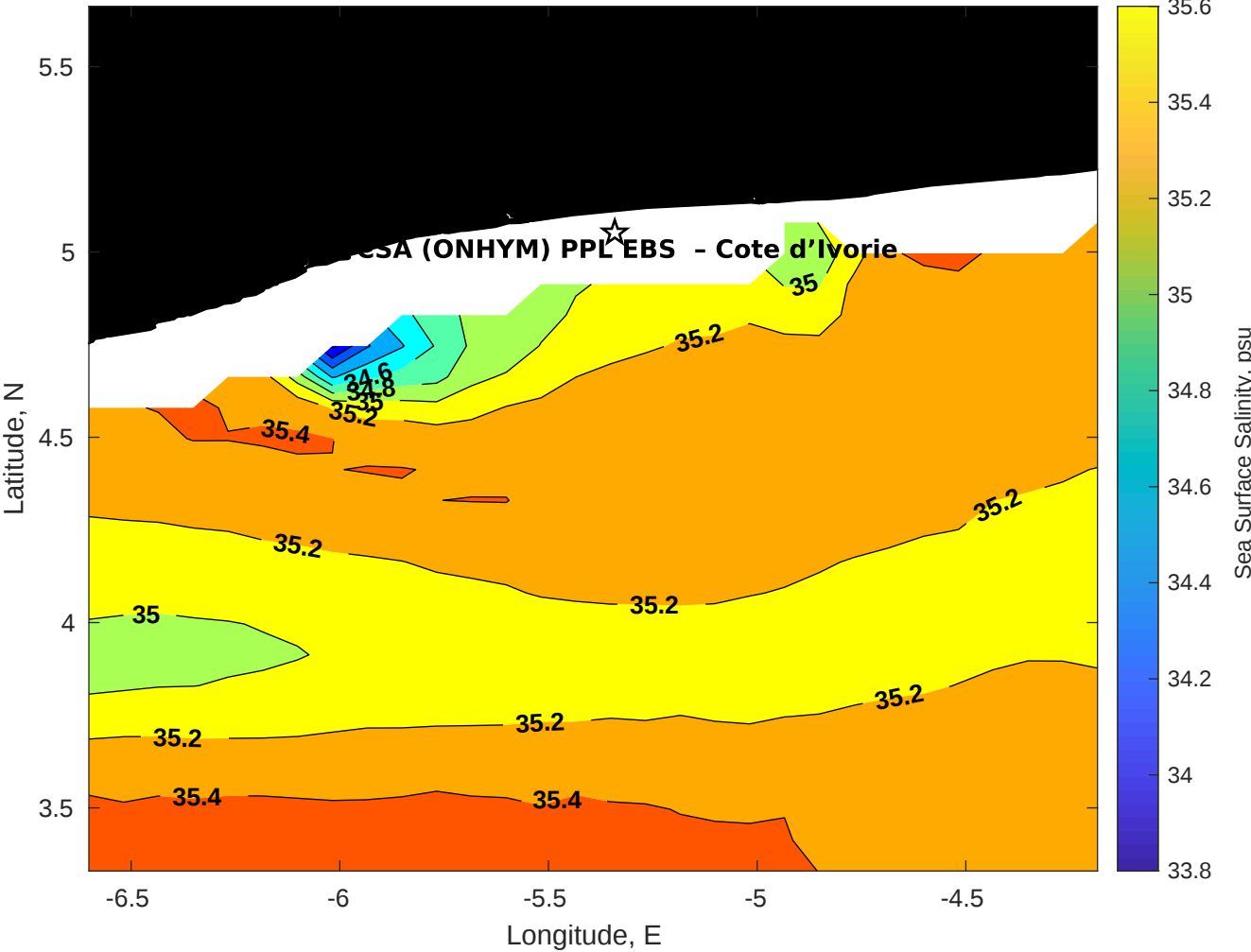
Surface Salinity for CSA (ONHYM) PPL EBS - Cote d'Ivoire at 29-Aug-2025 00:00:00
