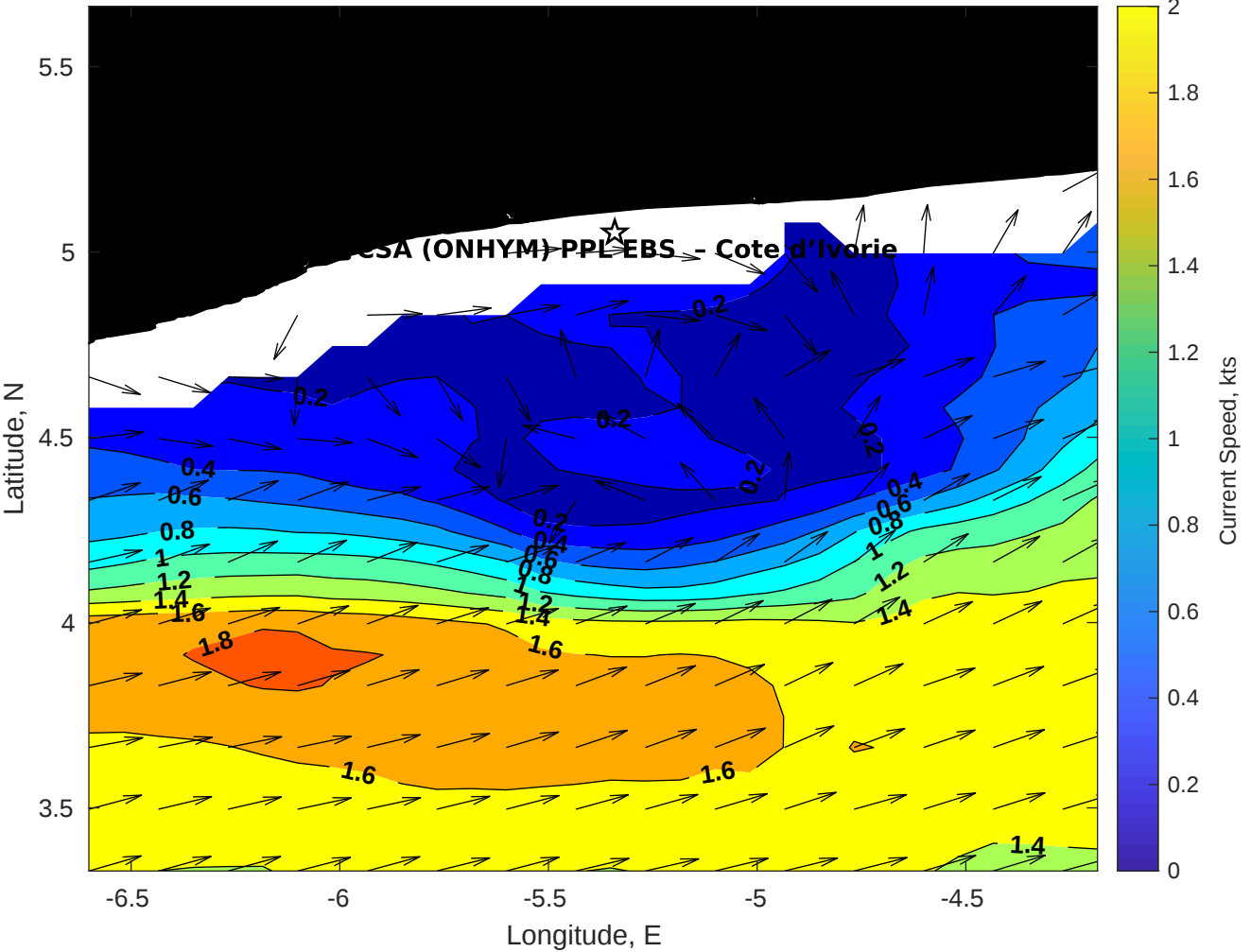
Surface Currents for CSA (ONHYM) PPL EBS - Cote d'Ivoire at 29-Aug-2025 00:00:00
