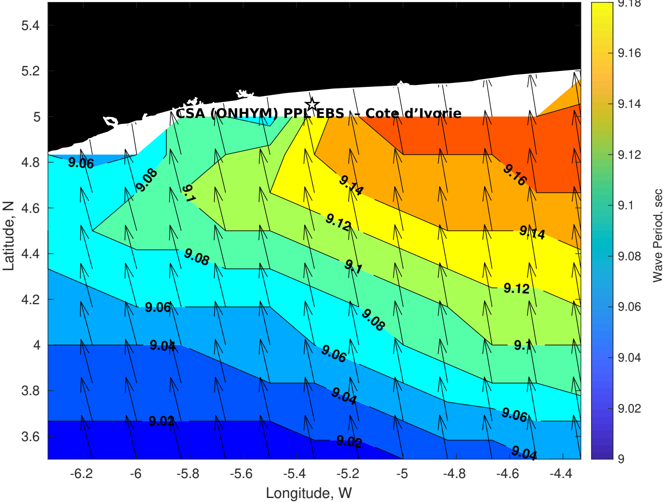
Wave Period (sec) for CSA (ONHYM) PPL EBS - Cote d'Ivoire at 30-Aug-2025 09:00:00
