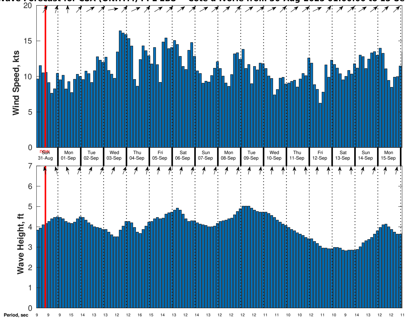
Wind & Wave Forecast for CSA (ONHYM) PPL EBS - Cote d'Ivoire from 30-Aug-2025 01:00:00 to 15-Sep-2025 01:00:00
