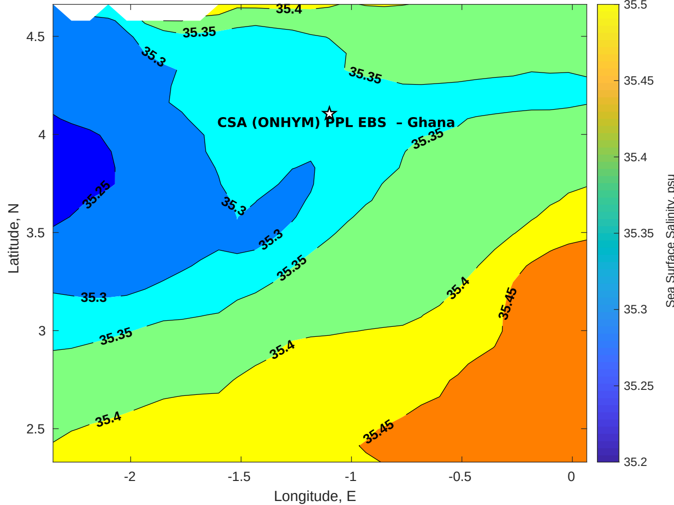
Surface Salinity for CSA (ONHYM) PPL EBS - Ghana at 29-Aug-2025 00:00:00
