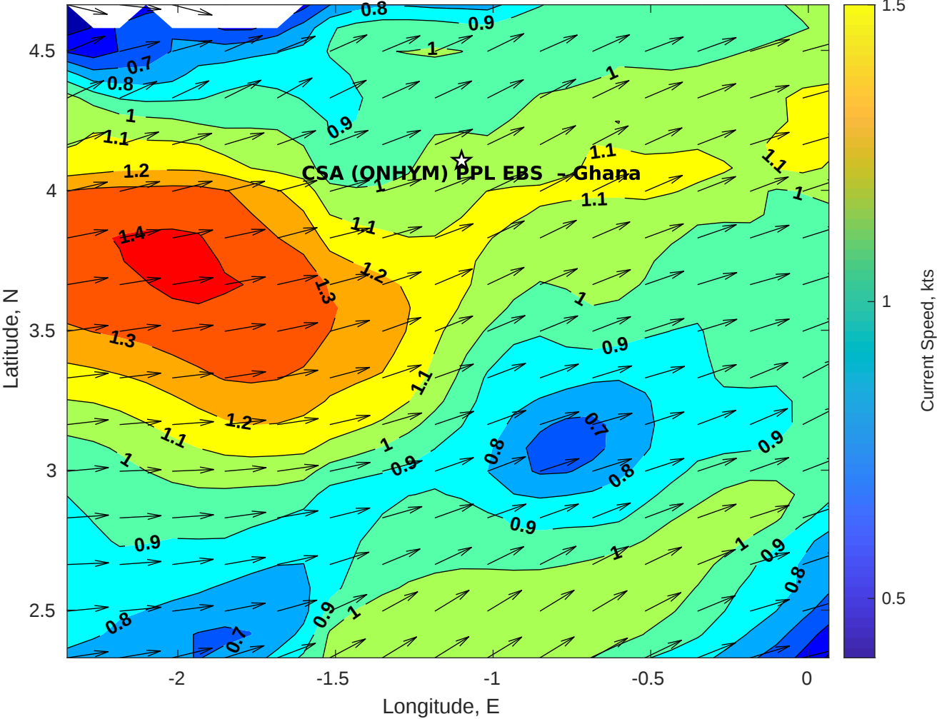
Surface Currents for CSA (ONHYM) PPL EBS - Ghana at 29-Aug-2025 00:00:00
