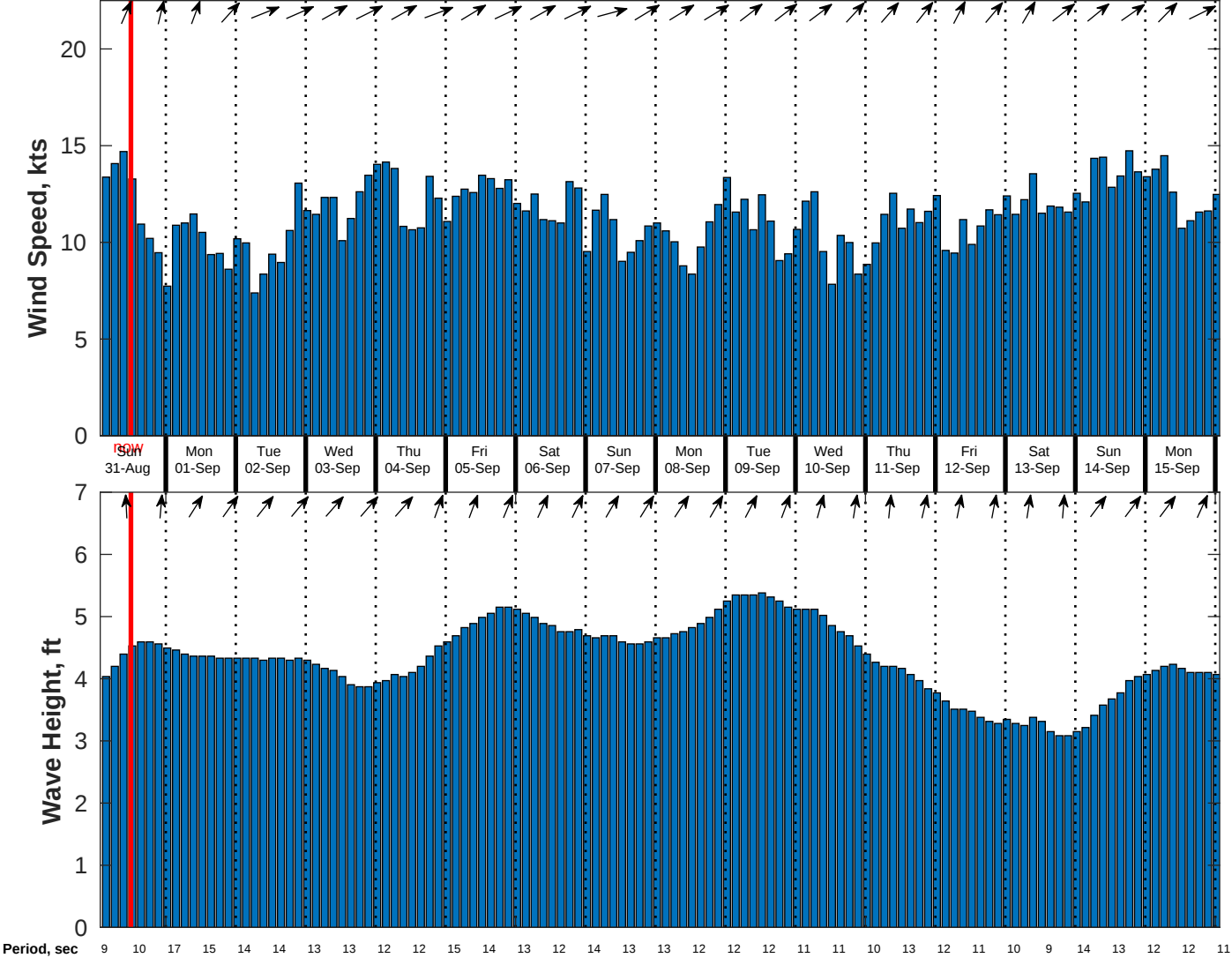
Wind & Wave Forecast for CSA (ONHYM) PPL EBS - Ghana from 30-Aug-2025 02:00:00 to 15-Sep-2025 02:00:00
