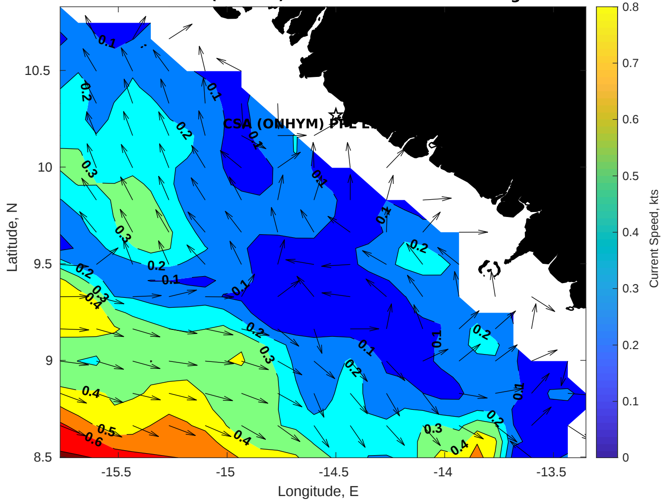
Surface Currents for CSA (ONHYM) PPL EBS - Guinea at 29-Aug-2025 00:00:00
