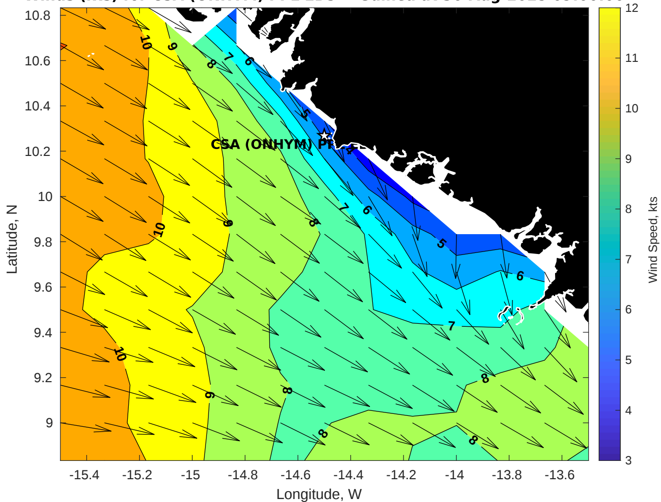
Winds (kts) for CSA (ONHYM) PPL EBS - Guinea at 30-Aug-2025 09:00:00
