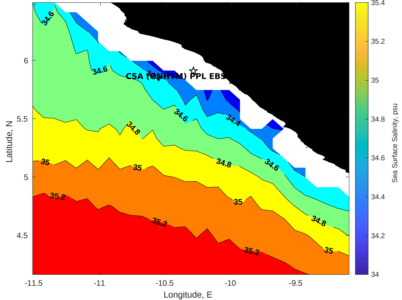
Surface Salinity for CSA (ONHYM) PPL EBS - Liberia at 29-Aug-2025 00:00:00
