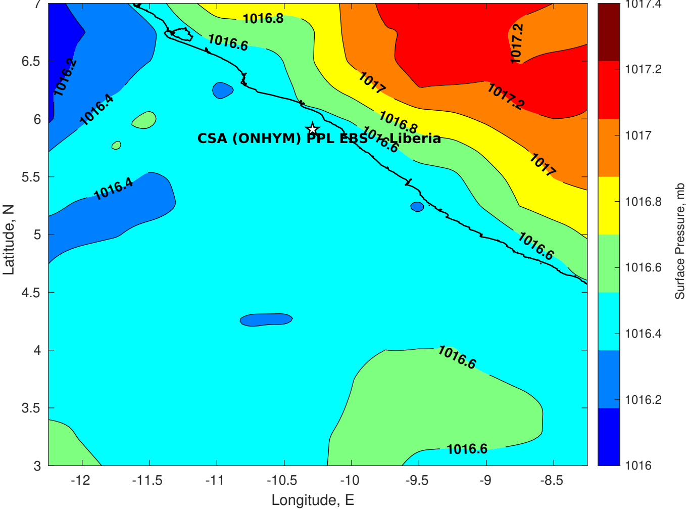
Surface Pressure (mb) for CSA (ONHYM) PPL EBS - Liberia at 01-Sep-2025 00:00:00
