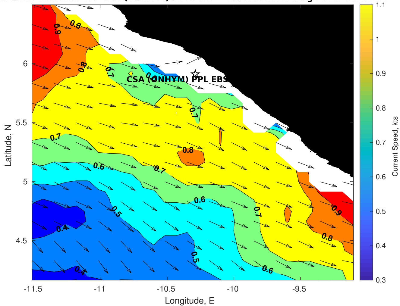
Surface Currents for CSA (ONHYM) PPL EBS - Liberia at 29-Aug-2025 00:00:00
