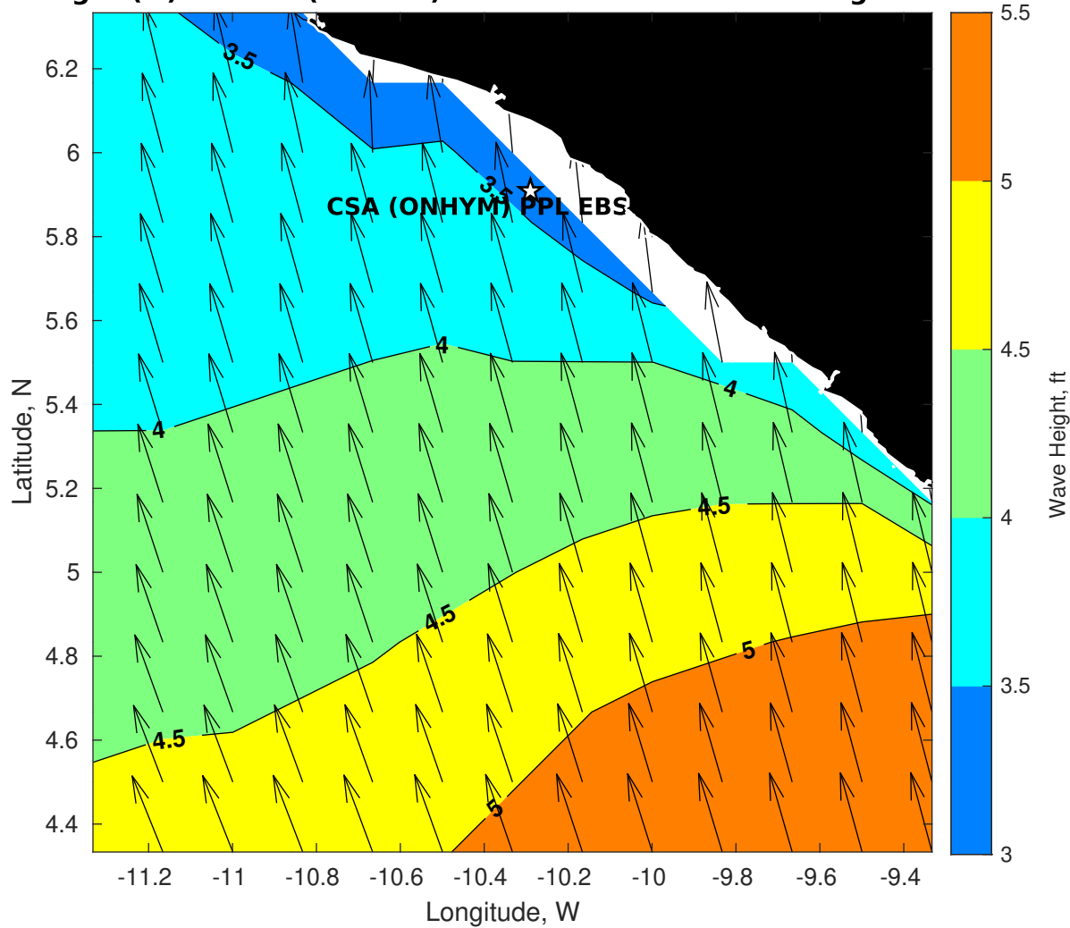
Wave Height (ft) for CSA (ONHYM) PPL EBS - Liberia at 30-Aug-2025 09:00:00
