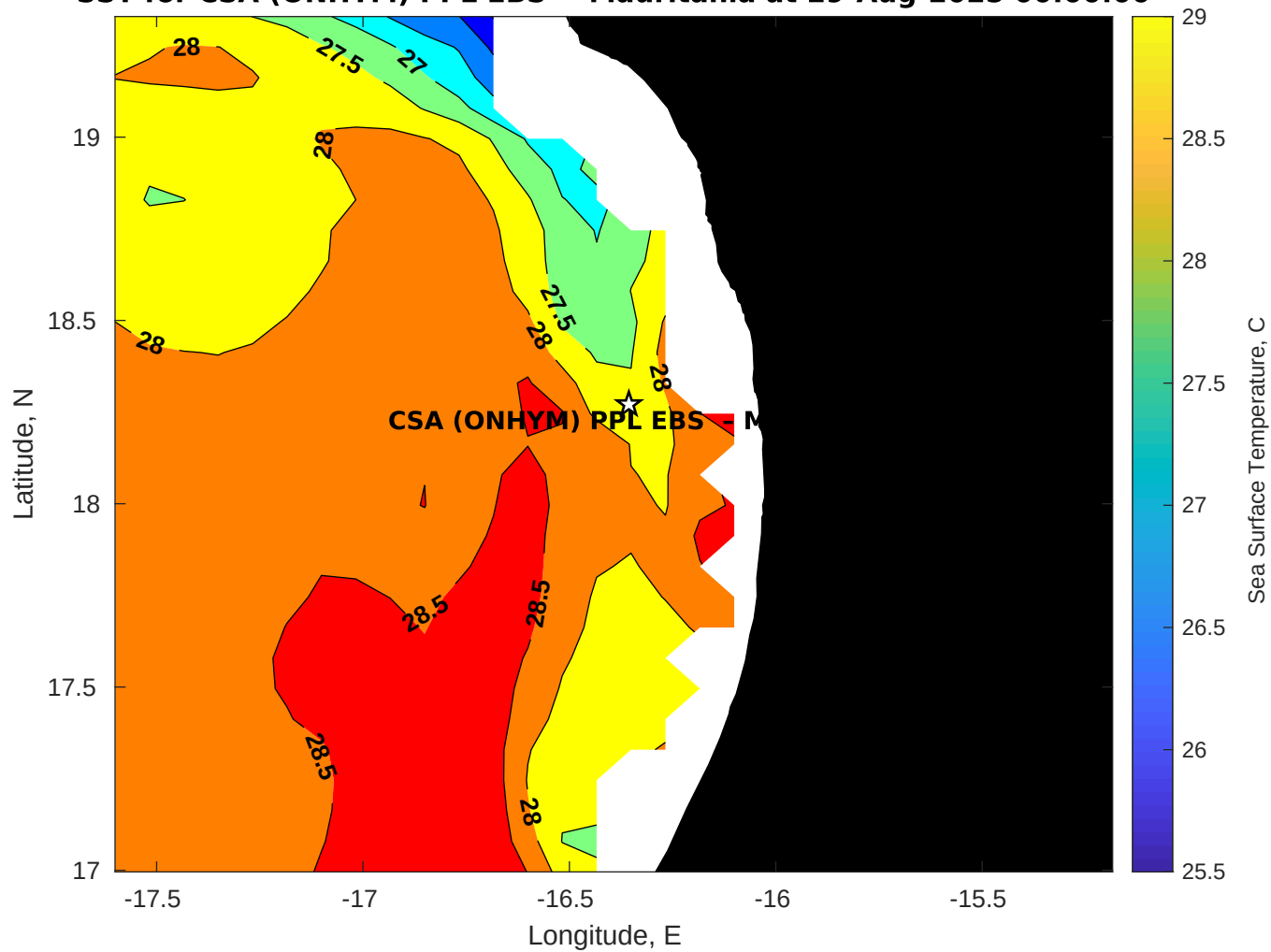
SST for CSA (ONHYM) PPL EBS - Mauritania at 29-Aug-2025 00:00:00
